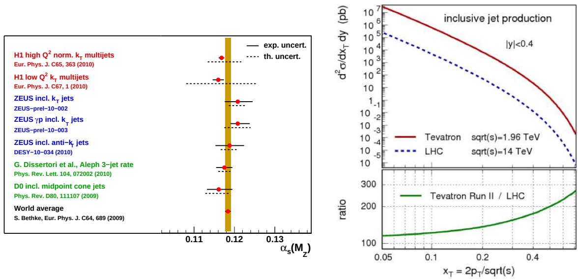
Figure 4. Examples of analyses of current HEP data with potential future impact. Left: Recent determinations of the strong coupling \alpha_s(M_Z) from a variety of experiments compared to the 2009 world average [25]. Right: A comparison of the predicted inclusive jet production cross sections at the Tevatron and the LHC, as a function of x_T [28].
