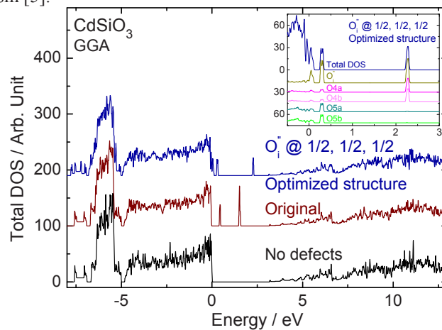
Fig. 5. Calculated (GGA method) density of states of the original and structure optimized \text{CdSiO}_3 with and without an interstitial oxide ion. Inset: Calculated total density and partial density of \text{O}_i'' and oxygen atoms in the O4 and O5 sites.
