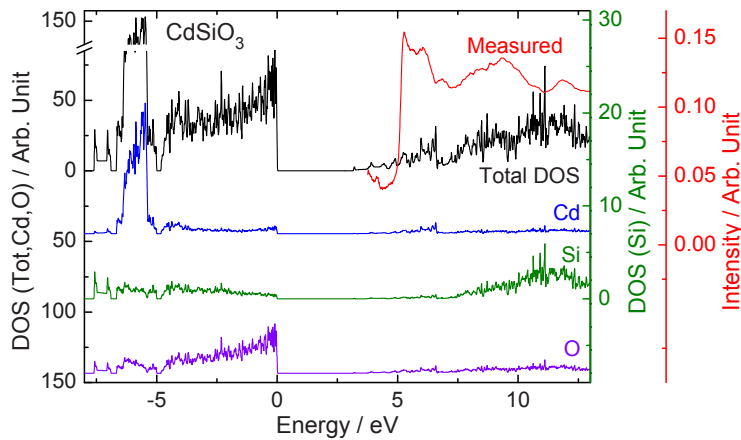
Fig. 4. Calculated (GGA method) density of states with the UV-VUV synchrotron radiation excitation spectrum of \text{CdSiO}_3 at 10 K ( \lambda_{\text{em}} : 600 nm).
