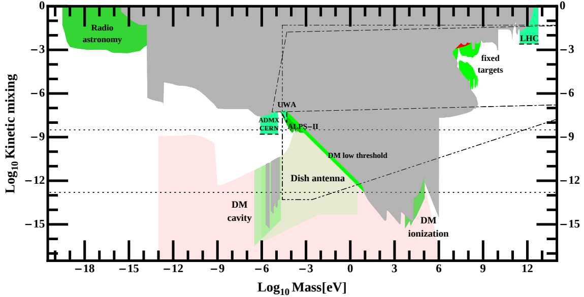
Fig. 3: Parameter space for hidden photons (HPs). The grey region indicates the parameter space already excluded by different experiments, see [3] for details. The reddish area in the bottom indicated the region in which HPs could constitute Cold Dark Matter. Various shades of green correspond to parameter regions accessible by planned and proposed experiments.
