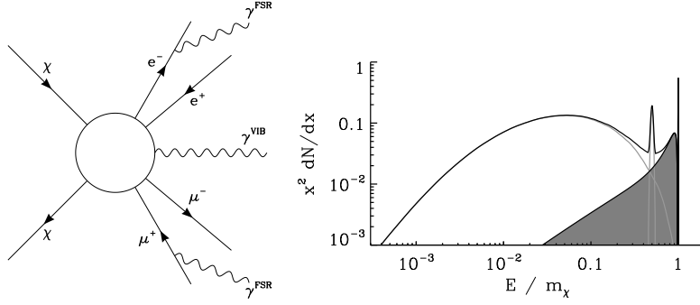
Line Signal (loop level \mathcal{O}(\alpha^2) )
