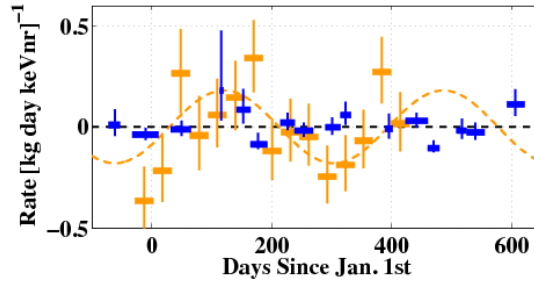
Figure 2.11: Contrast between the CDMS II and the CoGeNT annual modulation in the 5.0 – 11.9 keV nr range (the index nr standing for nuclear recoil), after subtracting the best fit unmodulated rate for each detector. The blue points show the rate of the CDMS II nuclear-recoil band, starting in late 2007. The orange points show the derived CoGeNT rate for nuclear recoils, starting in 2009. The orange dashed line shows the maximum-likelihood modulation model for the corresponding energy range. The CDMS II band is consistent with no modulation while the CoGeNT collaboration has reported a modulation in the electron-recoil band. Figure from Ahmed et al. [2012] and references therein.
