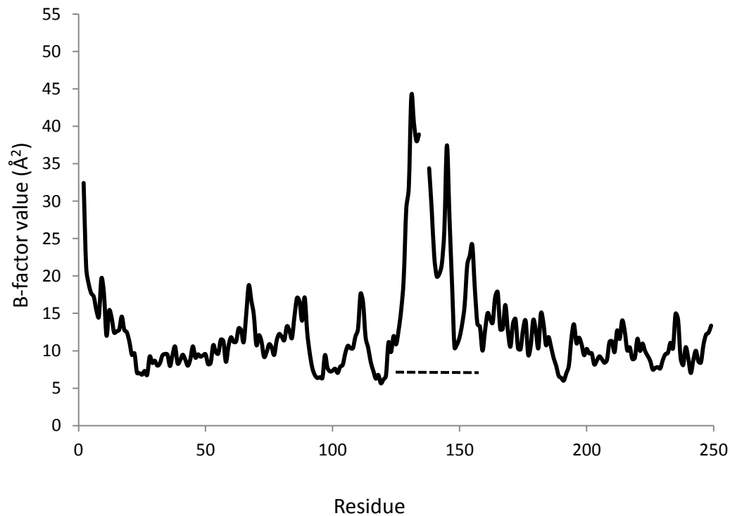
Figure S2: Graph showing the B-factor values of Ca atom of each amino acid of bMGL; the dotted line indicates the cap region of bMGL (Ile119-Thr164)
