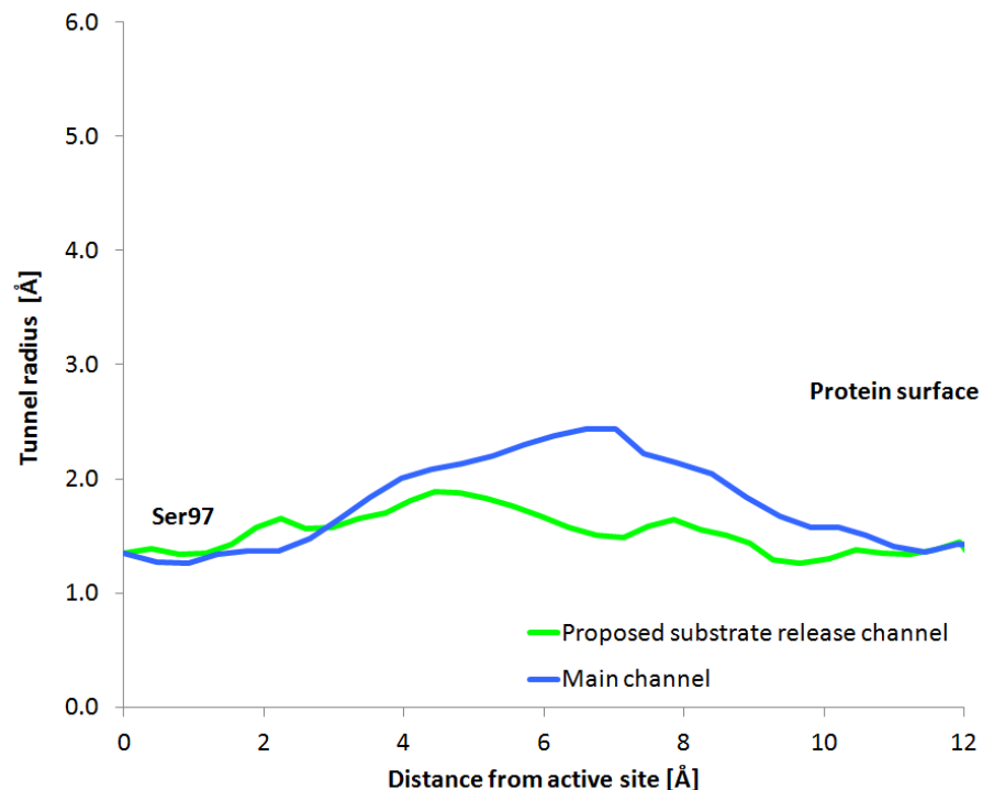
A) bMGL_80 ns MD; closed conformation
