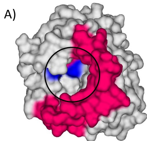
bMGL open, (PDB: 3RM3)
