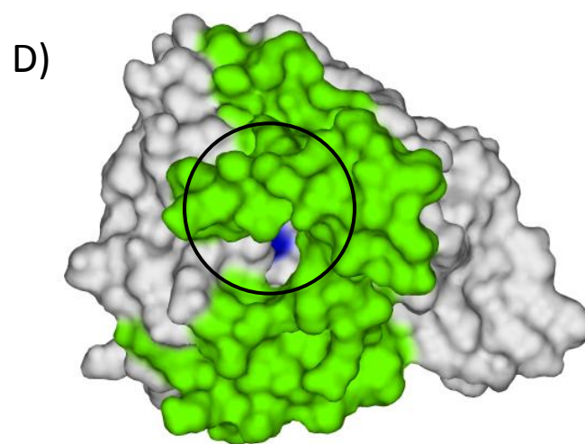
hMGL closed , (PDB: 3PE6)
