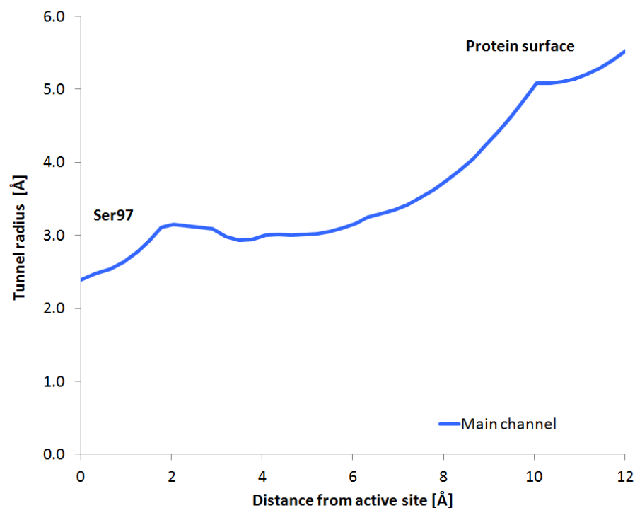
B) bMGL_80 ns MD; open conformation
