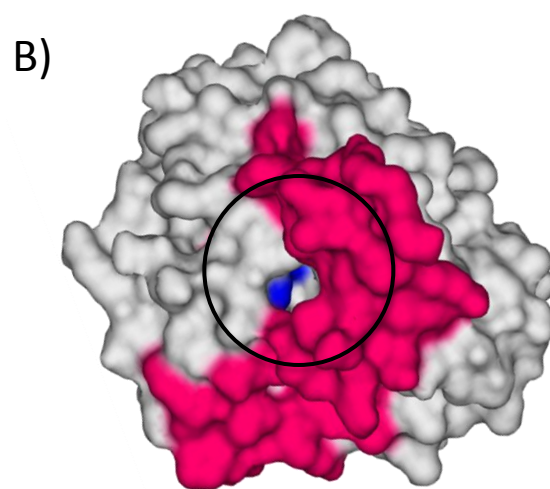
bMGL after MD Simulation for 100ns
