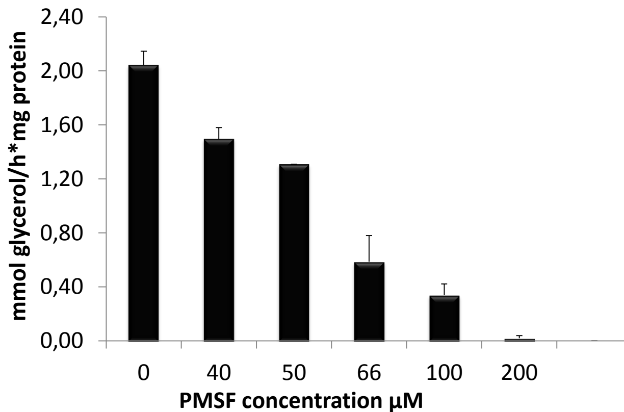
Figure S4: Inhibition of bMGL with increasing concentrations of PMSF. X-axis shows the concentration of PMSF and Y-axis the corresponding specific activity of bMGL.
