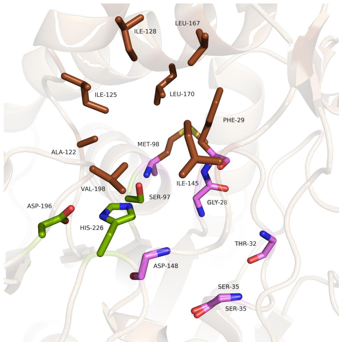
Figure S3: Atomic details of the hydrophobic and hydrophilic regions of the substrate binding pocket of bMGL. The hydrophobic residues are coloured brown, hydrophilic pink and the catalytic triad in green.
