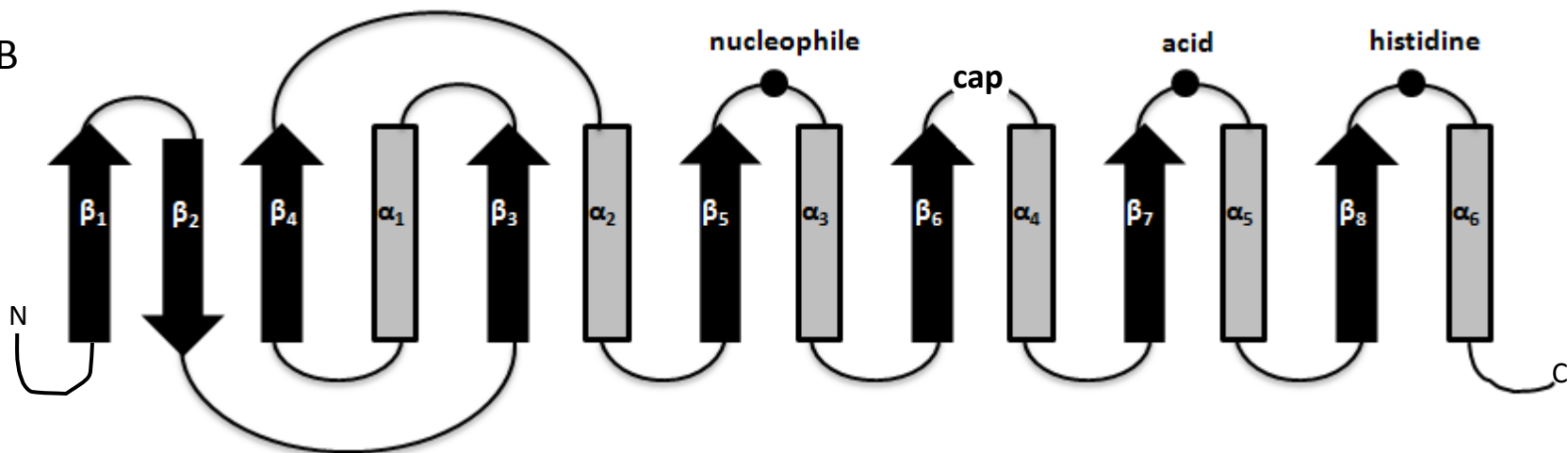
Figure S1: A) Schematic representation of minimal \alpha/\beta hydrolase fold observed in the structure of bMGL; B) Schematic representation of canonical \alpha/\beta hydrolase showing 8 backbone \beta strands and 6 \alpha helices; N and C represent the respective termini of the protein.
