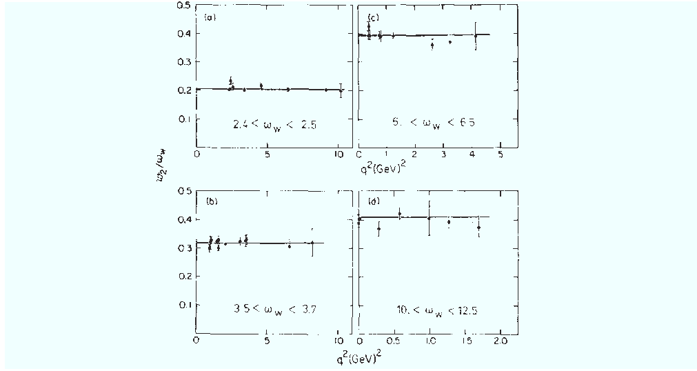
Figure 3: The function \nu W_2 plotted vs |q^2| assuming R = |q^2|/\nu^2 for different fixed \omega_W = (1/x + M_N^2/|q^2|)/(1 + 0.2/|q^2|) ; from [26] ©(1972) by Elsevier Science.
