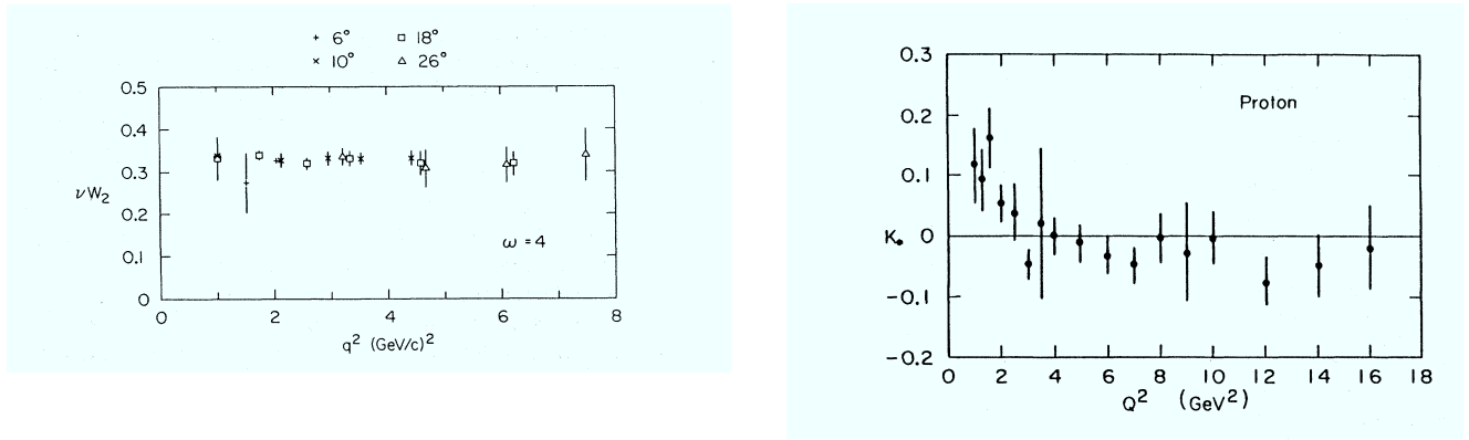
Figure 2: Left: An early observation of scaling: \nu W_2 for the proton as a function of -q^2 for W > 2 \text{ GeV} , at x = 1/\omega = 0.25 ; Right: The Callan-Gross relation: K_0 = F_2/(2xF_1) - 1 vs -q^2 . These results established the spin of the partons as 1/2; from [18], ©(1991) by the American Physical Society.
