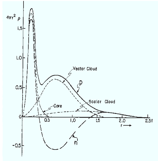
Figure 1: Charge distribution for the proton and the neutron implied by the form factors of Ref. [10], Figure 2(b); from [10], ©(1961) by the American Physical Society.
