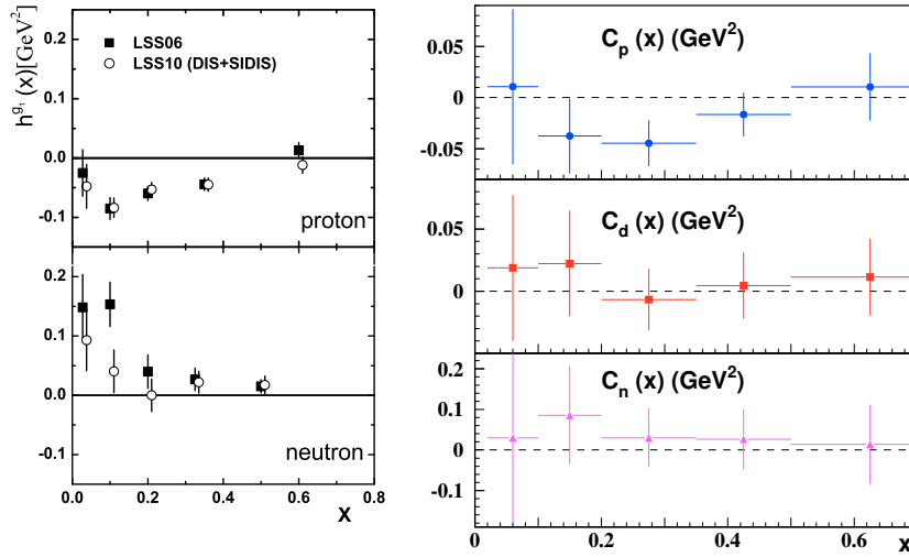
Figure 23: Left: comparison between the higher twist values corresponding to the fits of inclusive DIS LSS06 [456] and combined inclusive and SIDIS data set LSS10 [342] ©(2010) by the American Physical Society. Right: The additive higher twist coefficients C_p(x) , C_d(x) and C_n(x) [329], ©(2010) by Elsevier Science.
