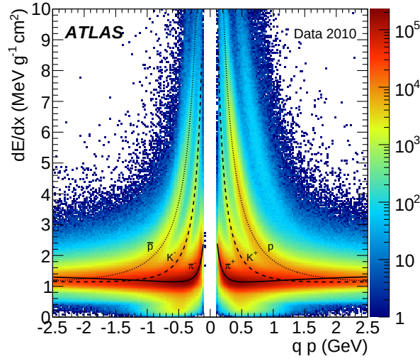
Figure A.8: Coloured version of Figure 1 (left): Distribution of dE/dx versus charge times momentum for minimum bias collisions in a data sample from 2010. With tracks reconstructed for p_T > 100 MeV this sample is more suitable for the calibration of the Bethe-Bloch function than 2011 data in which tracks had a cutoff of p_T = 400 MeV. The distribution of the most probable value for pions (solid), kaons (dashed) and protons (dotted) are superimposed.
