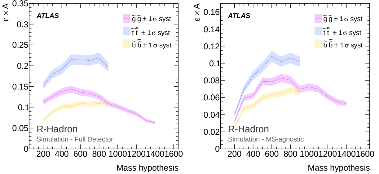
Figure A.15: Efficiency times acceptance for the tested R -hadron mass hypotheses. Each point on the x-axis represent a hypothesis mass, the efficiency for a given hypothesis is based on the number of signal events in the counting region after cuts, divided by the number of generated events. The band represents the 11.4% systematic uncertainty on the efficiency.
