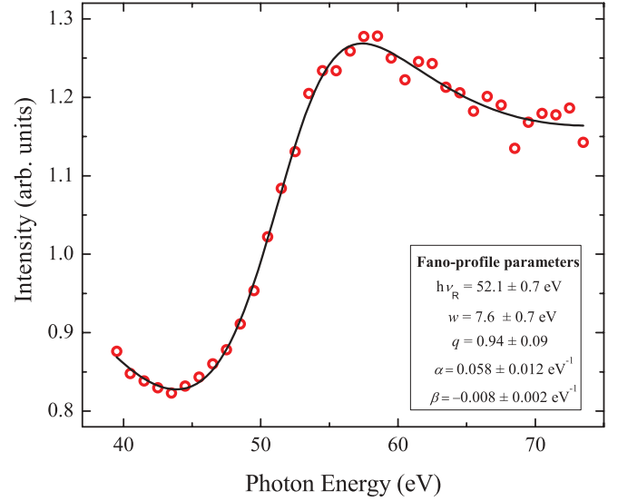
FIG. 7. (Color online) Fano resonance of the Ru 4d states gap ( E_F - 7.8 eV) calculated from the spectra presented in Fig. 4(c).
