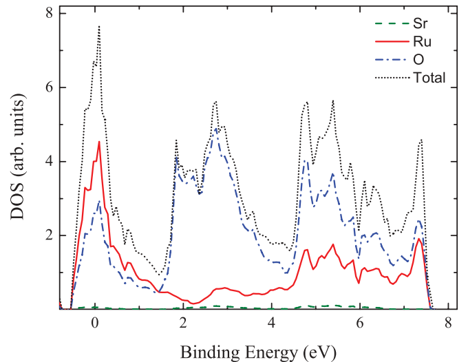
FIG. 5. (Color online) The total and partial DOS of \text{SrRuO}_3 calculated using the PBE exchange-correlation functional. The Fermi energy is set at zero.
