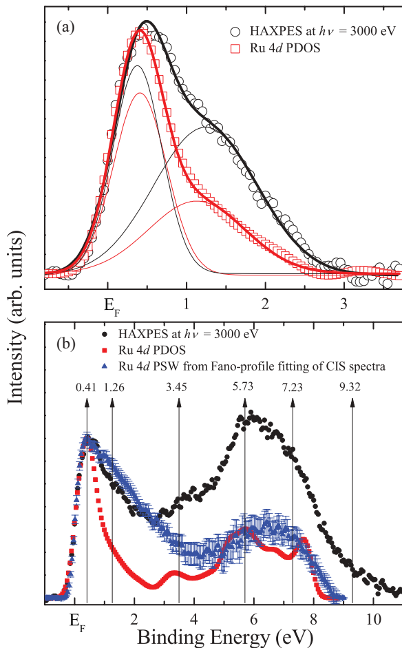
FIG. 14. (Color online) (a) Comparison of convoluted DFT results with the spectrum measured at h\nu = 3000 in the dominant Ru 4 d region (see Fig. 12). Thin lines represent the spectral components and thick lines are the spectral envelopes. (b) Comparison of VB spectra measured at h\nu = 3000 eV with the Ru 4 d PSW extracted from resonant UPS measurements and the convoluted DFT results. Arrows represent the positions of spectral components (in eV) obtained by fitting cumulative HAXPES spectra at h\nu = 3000 eV. Error bars show the confidence interval at 95% level, i.e., twice the standard error.
