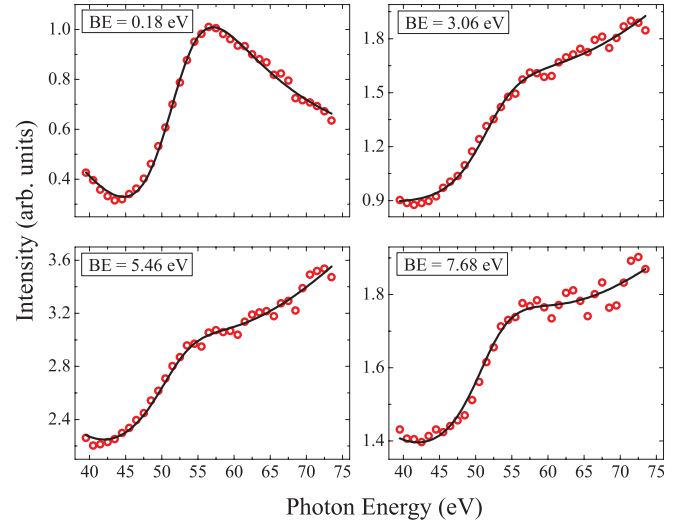
FIG. 9. (Color online) The Fano-profile CIS spectra of \text{SrRuO}_3 thin film measured at BE corresponding to the second derivative minima in the EDC spectra [see Fig. 4(b)].
