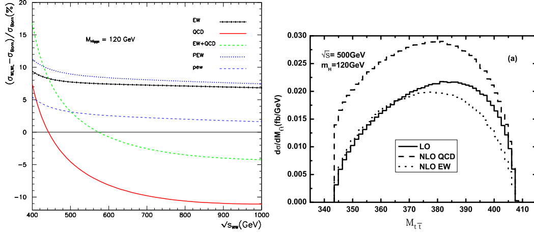
Figure 2: Left: relative NLO corrections for the process WW \rightarrow t\bar{t} : the dashed green line are the full corrections, the black line the EW and the red the QCD corrections, respectively. Right: The t\bar{t} invariant mass distribution at LO (dark line), the dashed line gives the NLO QCD corrections, while the dotted one shows the NLO EW corrections.
