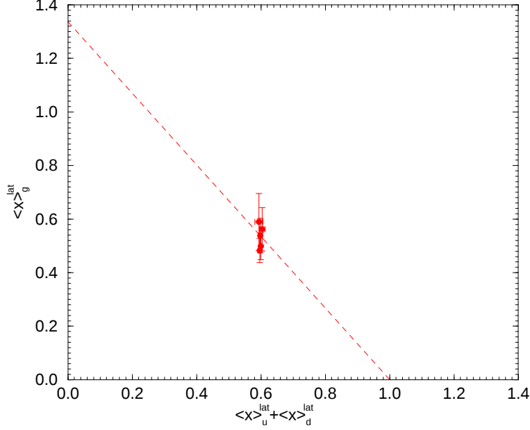
Figure 2: \langle x \rangle_u^{lat} + \langle x \rangle_d^{lat} against \langle x \rangle_g^{lat} for the five \kappa values, together with the line y = (1 - x)/0.748 .
