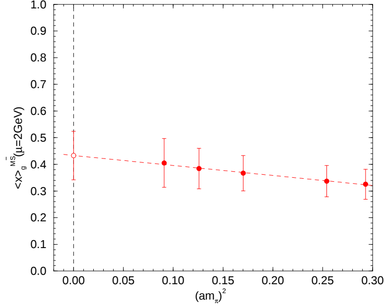
Figure 3: \langle x \rangle_g^{\overline{MS}}(\mu = 2 \text{ GeV}) versus (am_\pi)^2 for the five \kappa values, together with a linear chiral extrapolation.
