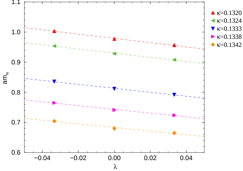
Figure 1: The nucleon mass against \lambda for the five \kappa values, together with a linear fit for each \kappa value.
