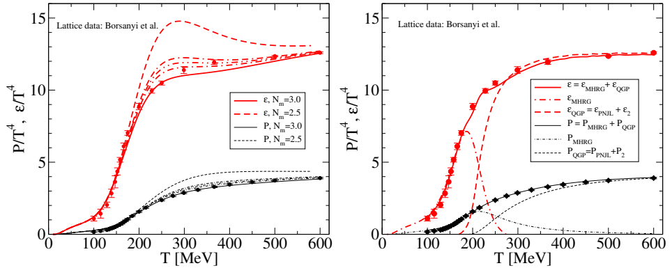
Fig. 1. Left: Thermodynamic quantities for the old Mott–Hagedorn Resonance Gas model [5]. Different line styles correspond to different values for the parameter N_m in the range from N_m = 2.5 (dashed line) to N_m = 3.0 (solid line). Lattice QCD data are from Ref. [1]. Right: Thermodynamic quantities for the new Mott–Hagedorn Resonance Gas, where quark-gluon plasma contributions are described within the PNJL model including \alpha_s corrections (dashed lines). Hadronic resonances are described within the resonance gas with finite width, as an implementation of the Mott effect (dash-dotted line). The sum of both contributions (solid lines) is shown for the energy density (thick lines) and pressure (thin lines) in comparison with the lattice data from [1].
