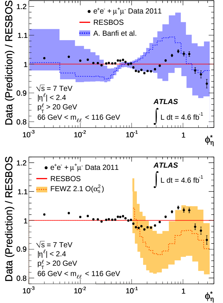
Figure 2: The ratio of the combined normalised differential cross section 1/\sigma^{\text{fid}} \cdot d\sigma^{\text{fid}}/d\phi_\eta^* to RESBOS predictions as a function of \phi_\eta^* . The inner and outer error bars on the data points represent the statistical and total uncertainties, respectively. The uncertainty due to QED FSR is included in the total uncertainties. The measurements are also compared to predictions, which are represented by a dashed line, from Ref. [22] and from FEWZ in the top and bottom panels, respectively. Uncertainties associated with these two calculations are represented by shaded bands. The prediction from FEWZ is only presented for \phi_\eta^* > 0.1 .
