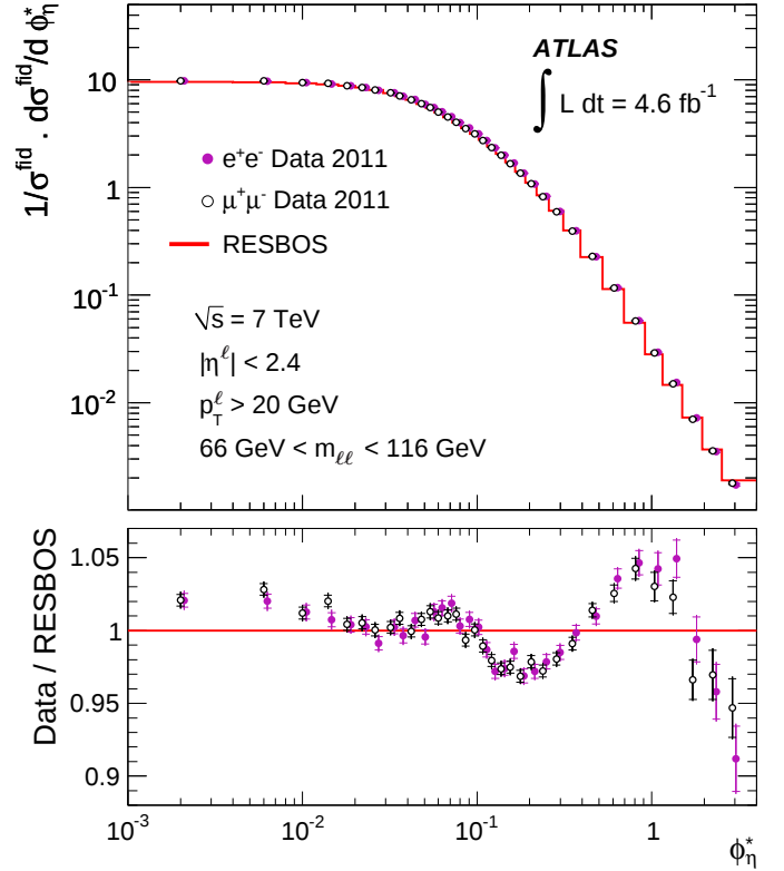
Figure 1: The measured normalised differential cross section 1/\sigma^{\text{fid}} \cdot d\sigma^{\text{fid}}/d\phi_\eta^* as a function of \phi_\eta^* for Z/\gamma^* \rightarrow e^+e^- (closed dots) and Z/\gamma^* \rightarrow \mu^+\mu^- (open dots) channels. The measurements are compared to RESBOS predictions represented by a line. The ratio of measured cross sections to RESBOS predictions is presented in the bottom panel. The measurements are displaced horizontally for better visibility. The inner and outer error bars on the data points represent the statistical and total uncertainties, respectively. The uncertainty due to QED FSR is included in the total uncertainties.
