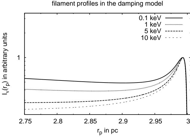
Fig. 3. Non-thermal X-ray intensity as a function of the projected radius calculated for four different X-ray energies with the parameters of Tycho given in Table 1, as well as l_d = 0.008 pc and B_{\max} = 85 \mu\text{G} . The forward shock is located at r_s = 3 pc.
