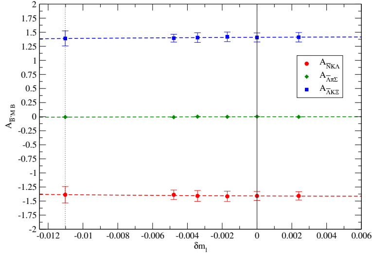
Figure 4: The matrix elements A_{\bar{N}K^0\Lambda} (red filled circles), A_{\bar{\Lambda}\pi^0\Sigma} (green filled diamonds) and A_{\bar{\Lambda}K^0\Xi} (blue filled squares) against \delta m_l , together with a quadratic fit.
