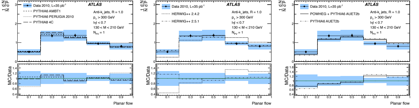
FIG. 9. The jet planar flow distributions for high mass ( 130 < M < 210 GeV), leading p_T , anti- k_t R = 1.0 jets in N_{PV} = 1 events, corrected to particle level.
