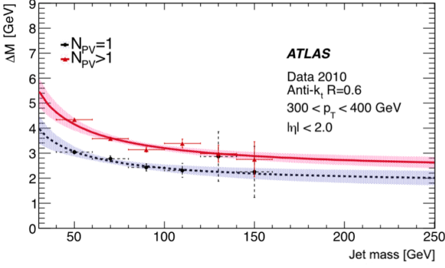
FIG. 2. The size of the mass shift in anti- k_t R = 0.6 jets with 300 < p_T < 400 GeV in jets with pileup and UE ( N_{PV} > 1 ) and with UE alone ( N_{PV} = 1 ). The curves are fits of the form \Delta M = p_{0_M} + \frac{p_{1_M}}{M} . The difference between the curves gives the contribution to the jet mass from pileup only. The 1\sigma uncertainties on the fits are shown in the error bands.
