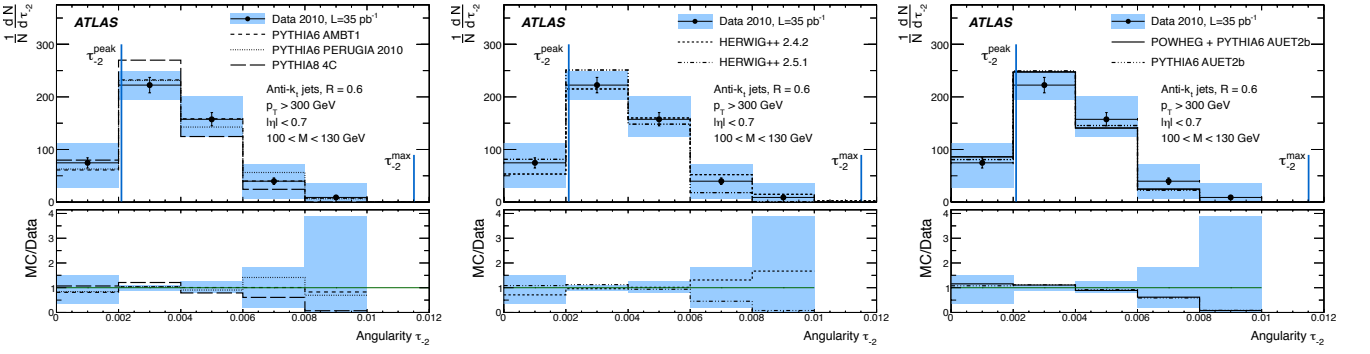
FIG. 10. The angularity \tau_{-2} distributions for leading p_T , anti- k_t R = 0.6 jets in the mass range 100 < M < 130 GeV, in the full 2010 data set, corrected to particle level. The peak and maximum positions predicted by the small angle approximation of Eq. 10 are indicated.
