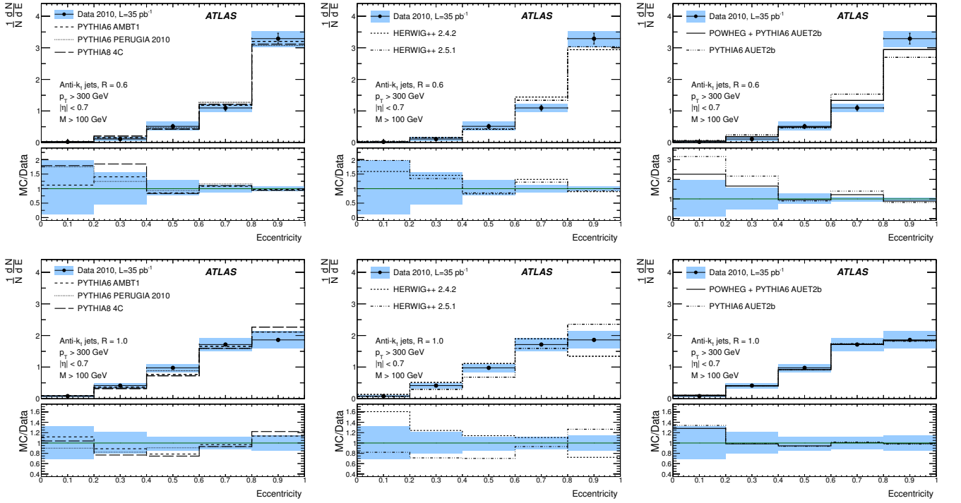
FIG. 8. The jet eccentricity distributions for high mass ( M > 100 GeV), leading p_T , anti- k_t R = 0.6 (top) and R = 1.0 (bottom) jets in the full 2010 data set, corrected for pileup and corrected to particle level.
