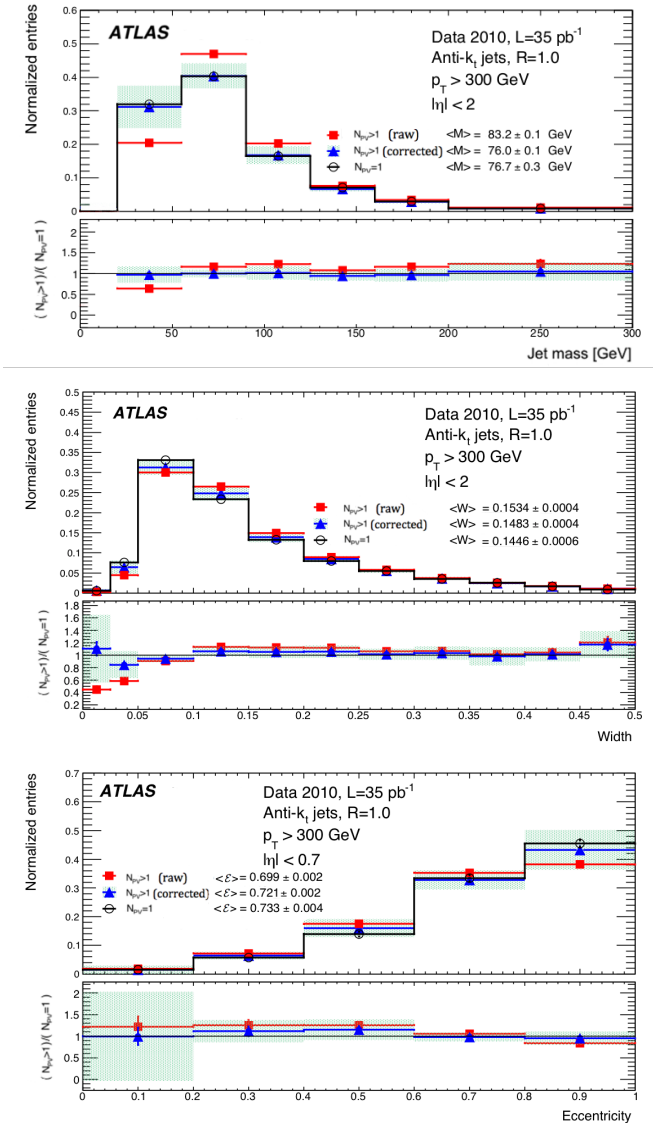
FIG. 3. The mass, width and eccentricity distributions before and after the pileup corrections. The (red) squares indicate the uncorrected data in the full data set, the (black) circles indicate the subset of this data with N_{PV} = 1 and the (blue) triangles indicate the full data set after pileup corrections. The mean value of each distribution is indicated in the legend with the corresponding statistical uncertainty. The lower region of each figure shows the measured ratio of N_{PV} > 1 to N_{PV} = 1 events.
