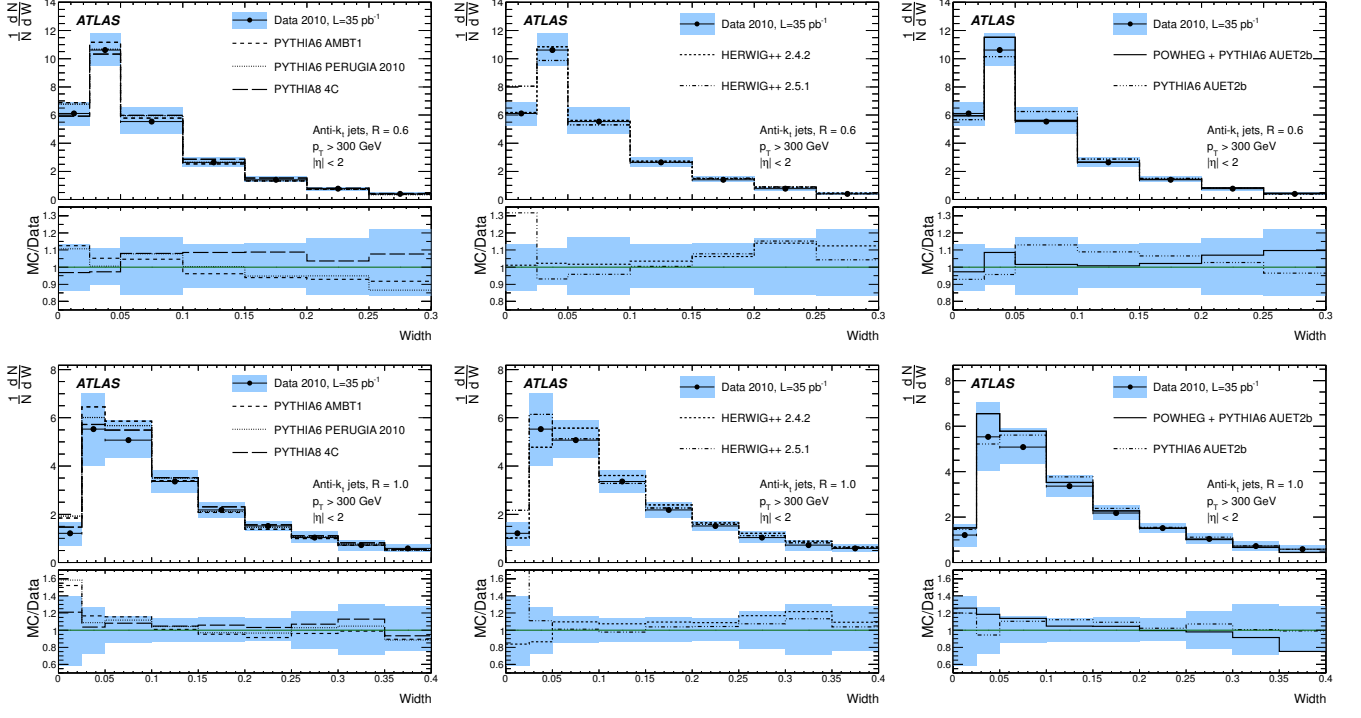
FIG. 7. The jet width distributions for leading p_T , anti- k_t R = 0.6 (top) and R = 1.0 (bottom) jets in the full 2010 data set, corrected for pileup and corrected to particle level.
