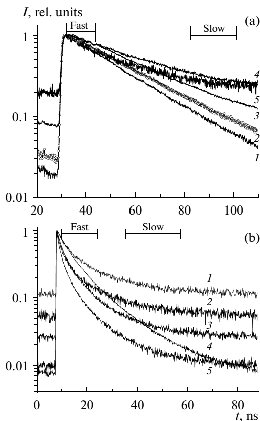
Fig. 3. PL decay curves of LaBr 3 –Ce for the PL excitation in (a) UV–VUV and (b) XUV spectral ranges at T = 295 K: (a) \lambda_{\text{rad}} = 356 nm and E_{\text{exc}} = (1) 4.27, 3.87, 4.6, (2) 4.86, (3) 5.52, (4) 6.88, and (5) 7.75 eV and (b) \lambda_{\text{rad}} = (1) and (2) 430 and (3)–(5) 356 nm and E_{\text{exc}} = (1) and (3) 130, (2) and (5) 118, and (4) 500 eV. Segments Fast and Slow show the time windows that correspond to the fast and slow components, respectively, in the time-resolved experiments.
