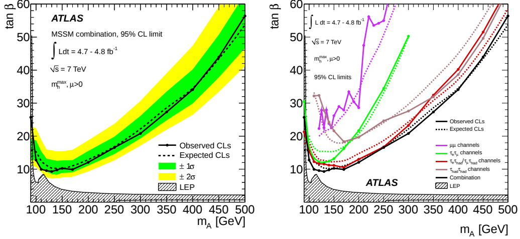
Figure 6. Expected (dashed line) and observed (solid line) 95% CL limits on \tan \beta as a function of m_A for the statistical combination of all channels along with the \pm 1\sigma and \pm 2\sigma bands for the expected limit are shown on the left plot. Values of \tan \beta greater than the shown lines are excluded. The 95% CL limits for the expected limit (dashed lines) and the observed limit (continuous lines) for each of the \mu\mu , \tau\tau , \tau_{lep}\tau_{had} and \tau_{had}\tau_{had} channels and their statistical combination are shown on the right plot. The 95% CL exclusion region from neutral MSSM Higgs boson searches performed at LEP[13] is shown in a hatched style.
