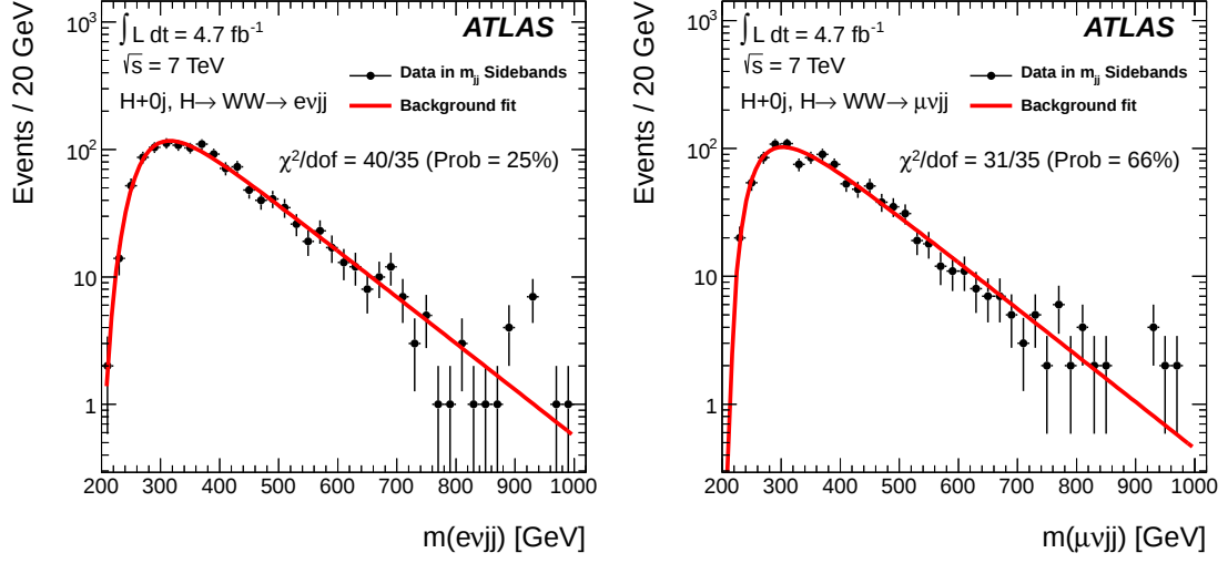
Figure 1: Fits of the background model described in the text to the reconstructed invariant mass m(\ell\nu jj) when m_{jj} is in the W sidebands for the \ell\nu jj + 0j selection. The left (right) figure shows the electron (muon) channel distribution. The \chi^2/\text{dof} and \chi^2 probability of these fits are also shown in the figure.
