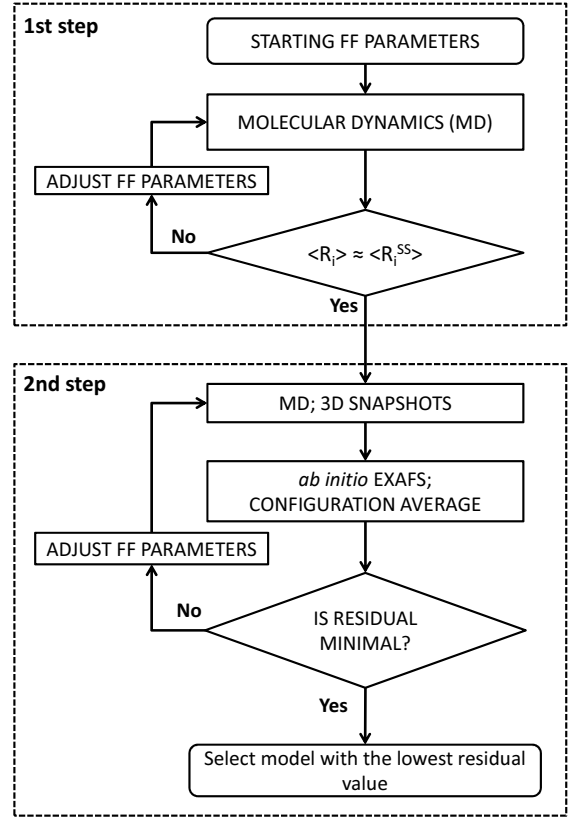
FIG. 6. A scheme of the MD-EXAFS calculation.
