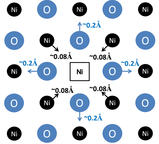
FIG. 8. (Color online) Schematic view of the nearest neighbor relaxation around nickel vacancy in the bulk of nickel oxide according to our molecular dynamics simulations. Note that oxygen atoms move outwards, but nickel atoms move inwards to the nickel vacancy.
