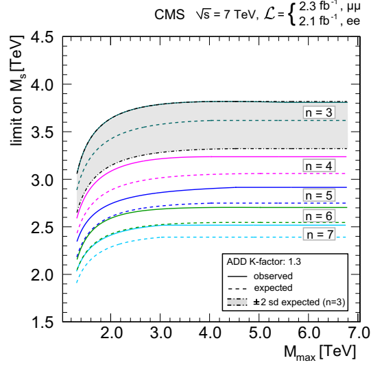
Figure 2: Observed and expected 95% CL lower limits on M_s , obtained by combining the \mu\mu ee results, for different numbers of extra dimensions n , applying a signal K-factor of 1.3. A confidence interval for the expected limit corresponding to 2 standard deviations (sd) is shown for the case n = 3 .
