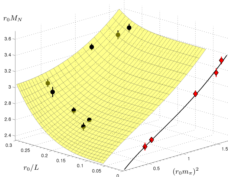
Figure 3: Fit (surface) to the nucleon mass data (full circles) for a range of r_0/L and (r_0 m_\pi)^2 values. Black circles lie above the surface, gray (or half gray) below (or on) the surface. The line and the red diamonds at r_0/L = 0 mark the fitted infinite volume prediction. For the sake of simplicity, for each (r_0 m_\pi)^2 only one extrapolated (red) point is shown at r_0/L = 0 .
