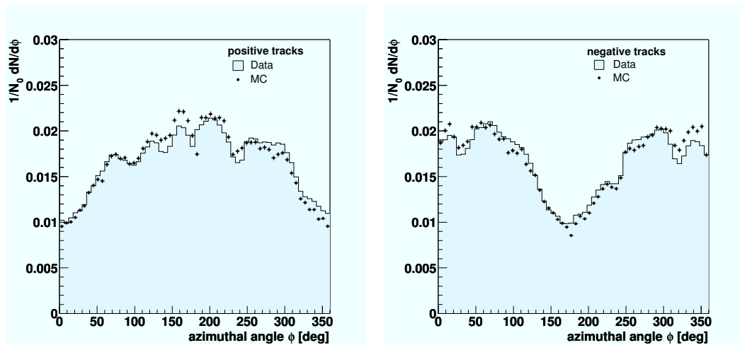
Figure 4.13: Distribution of the azimuthal track angle. The bending of the tracks in the magnetic field is clearly visible. All distributions are normalized to the same number of entries.
