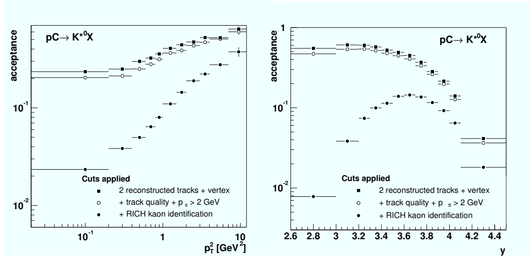
Figure 5.15: p_T^2 acceptance as a function of the different analysis cuts. Note that this plot was done using the Monte-Carlo track matching method.
