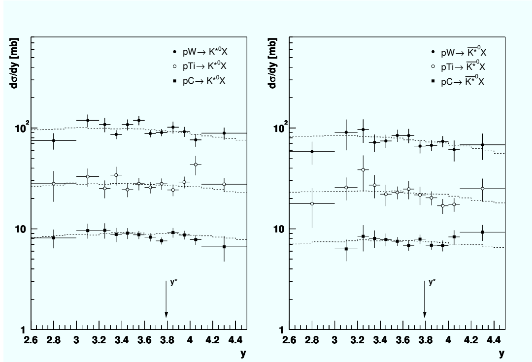
Figure 6.2: Inclusive differential cross sections d\sigma/dy for K^{*0} and \bar{K}^{*0} production at mid-rapidity. The dashed lines indicate the Monte-Carlo predictions.
