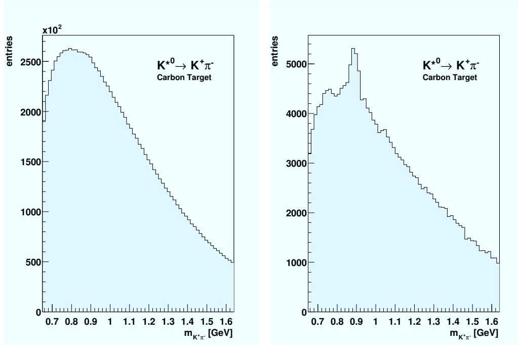
Figure 4.4: Invariant K^+\pi^- mass distributions in the region of the nominal K^{*0} mass. Left: Only event selection and vertex reconstruction applied. The K^{*0} signal is hidden by large combinatorial background. Right: After application of all selection cuts the background is reduced by a factor of about 60 and the K^{*0} signal is clearly visible.
