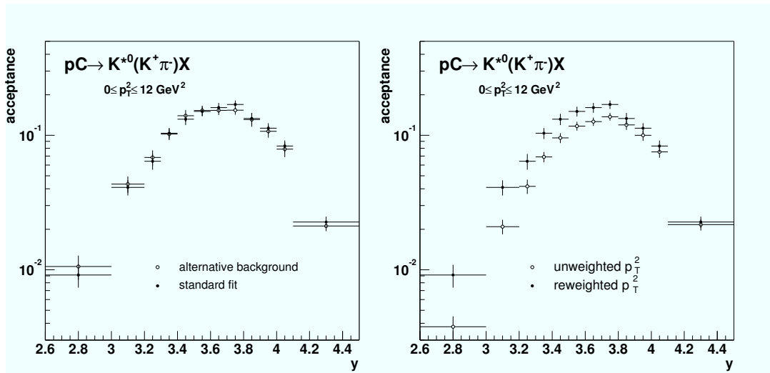
Figure 5.19: Comparison of the influence of different background parameterizations on the acceptance. Within the statistical errors no deviation is found.
