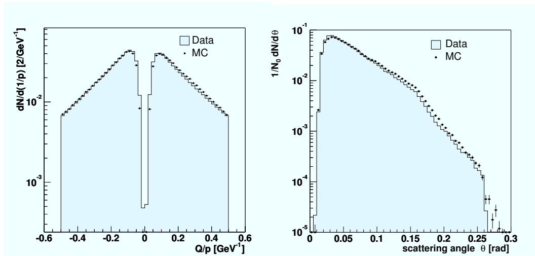
Figure 4.11: Q/p distribution for single tracks normalized to the same number of entries. The momentum cut at 2 GeV is clearly seen.
