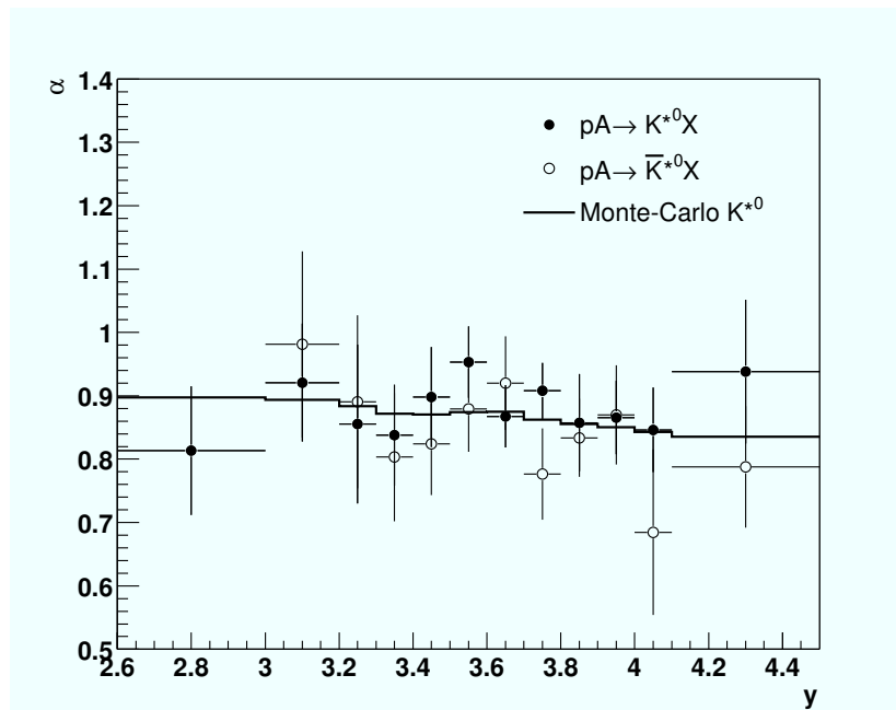
Figure 6.9: Atomic number dependence of the differential production cross sections as a function of rapidity.
