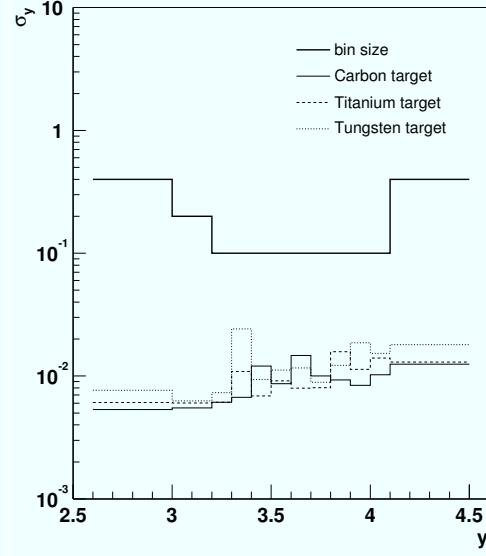
Figure 5.7: Same as in fig. 5.6 but for the rapidity distribution.
