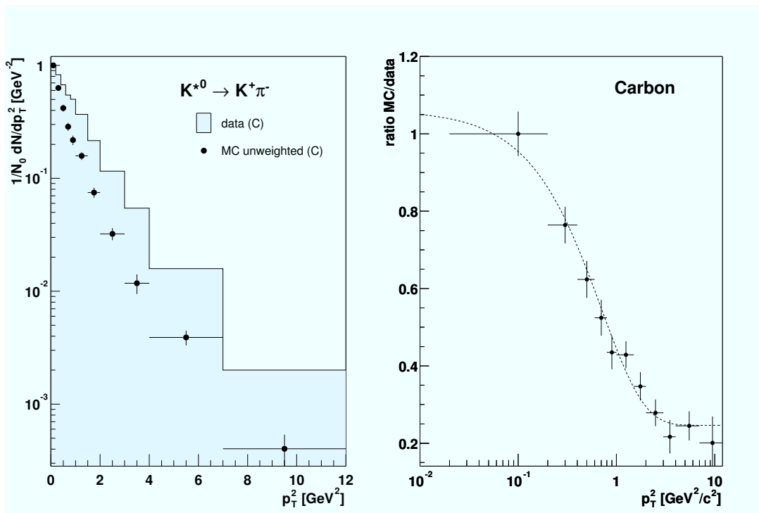
Figure 5.11: Comparison of uncorrected differential distributions in p_T^2 for data and Monte-Carlo before reweighting. The Monte-Carlo simulation underestimates the data significantly. The distributions are normalized to the first bin.
