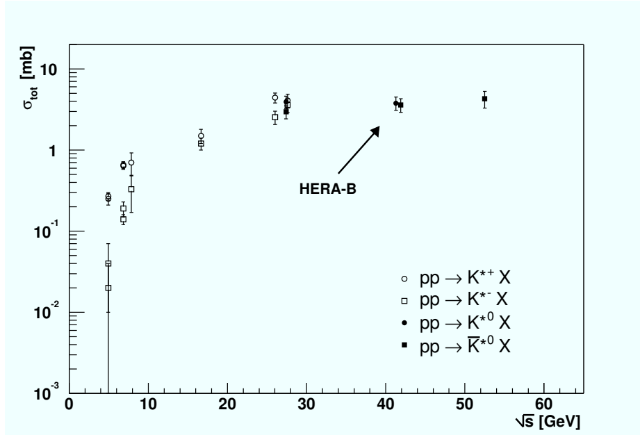
Figure 6.7: Comparison of K^* production cross sections at various center-of-mass energies [blo74, boc79, kic79, dri81, bri82, azi86, bog88, agu91]. The results of this analysis have been slightly displaced from each other for better visibility.
