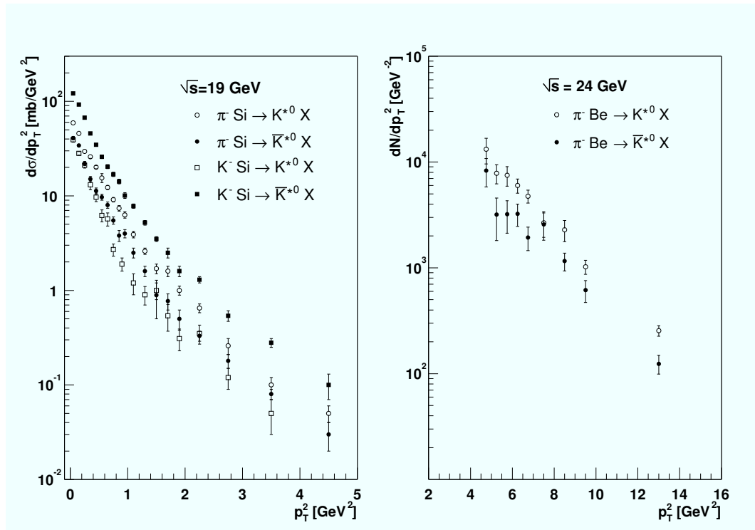
Figure 1.3: Transverse differential distributions for K^{*0} and \bar{K}^{*0} production on light nuclear targets. Left: Results of [faw90] for 200 GeV \pi^- and K^- beams interacting with a fixed silicon target. The acceptance of the measurement covers the full longitudinal phase space. Right: Measurements from [bel93] for a 300 GeV \pi^- beam incident on a beryllium target. The measurement was done at mid-rapidity. Note that this latter result does not include an absolute normalization.
