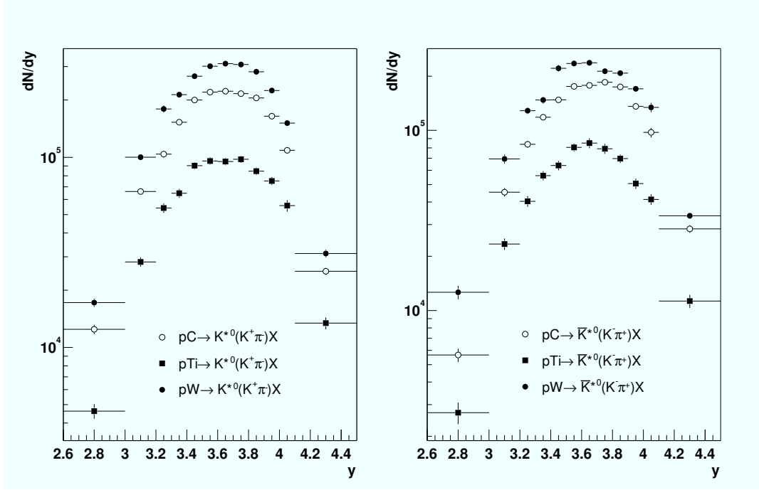
Figure 5.2: The uncorrected differential K^{*0} rapidity distributions. Signal yields are given per unit of rapidity. Errors are statistical only.
