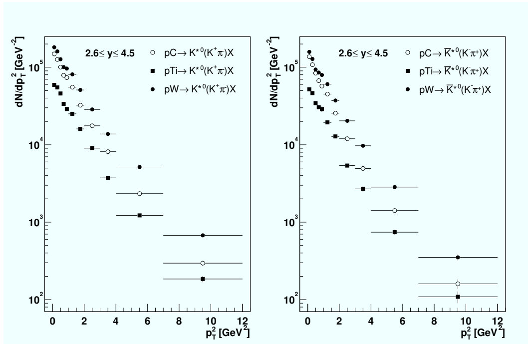
Figure 5.1: The uncorrected differential K^{*0} p_T^2 spectra. The errors are statistical only.
