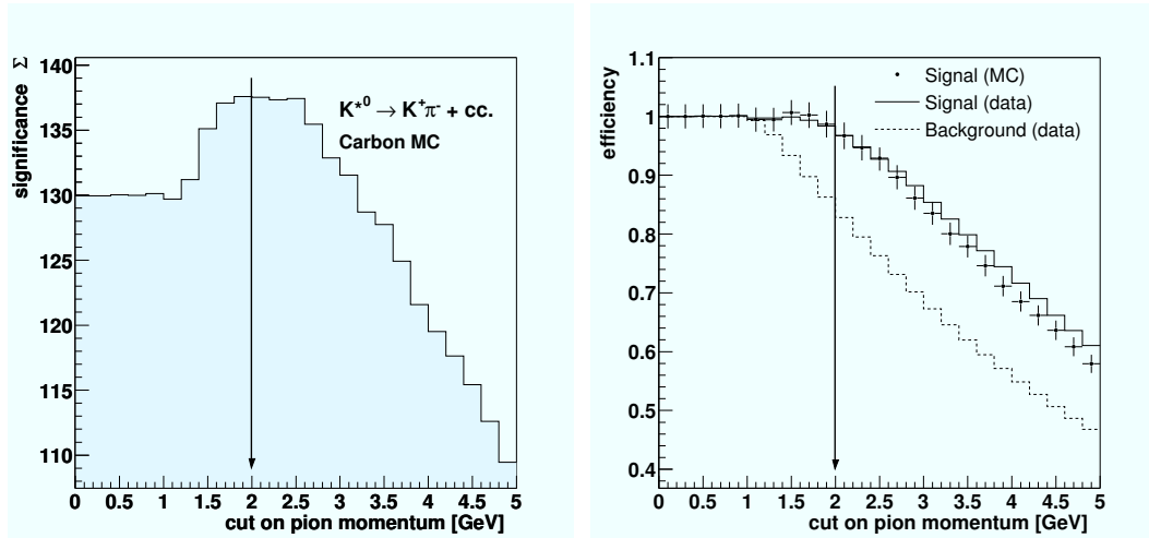
Figure 4.10: Left: Signal significance for carbon data as a function of the cut on the momentum of the pion candidate track. Right: Efficiencies of signal and background as a function of the cut. The dots with the error bars represent the signal efficiencies obtained from the Monte-Carlo.
