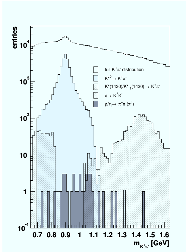
Figure 4.16: Expected contributions from resonances to the K^+\pi^- invariant mass distribution. To select the daughter tracks of the resonances, the Monte-Carlo track matching method is used.
