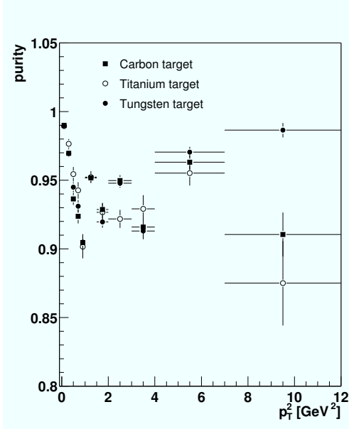
Figure 5.8: Bin purity as a function of the p_T^2 bin for the different data samples. See text for further explanation.
