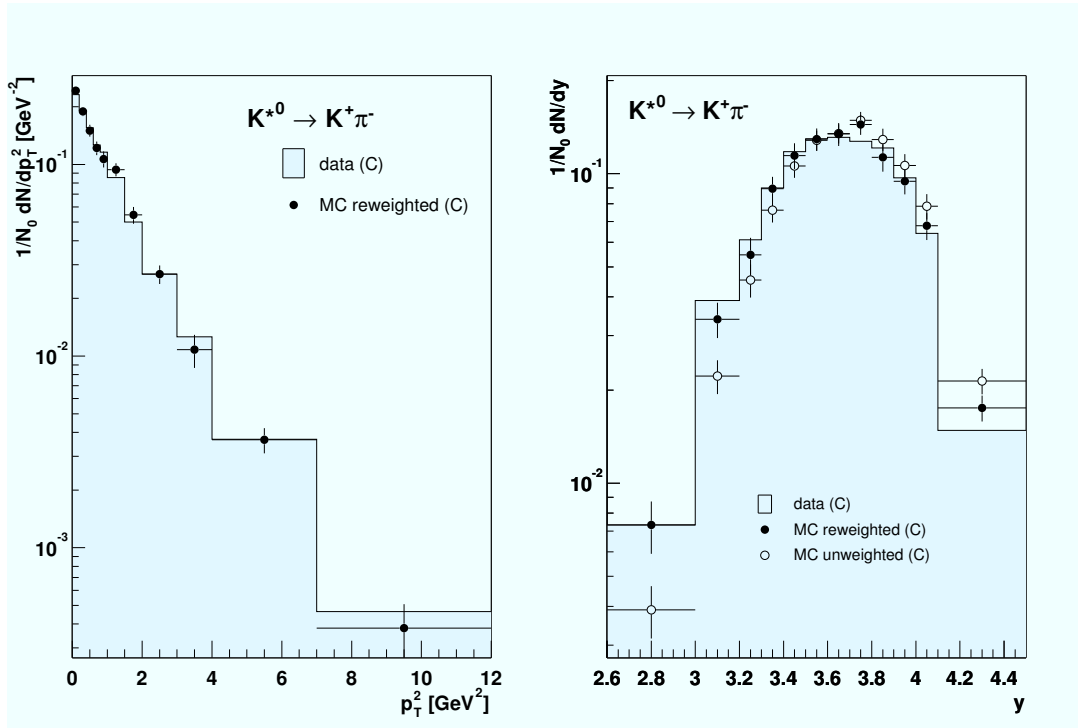
Figure 5.13: Uncorrected p_T^2 distributions for data and Monte-Carlo after reweighting. By construction, the Monte-Carlo reproduces the data. The distributions are normalized to the the same number of entries.
