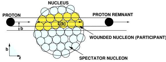
Figure 2.4: Schematic view of a proton-nucleus collision in the Glauber model. The projectile hits the nucleus with a certain impact parameter b . Only the nucleons along the projectile take part in the collision. Picture taken from [bru02].
