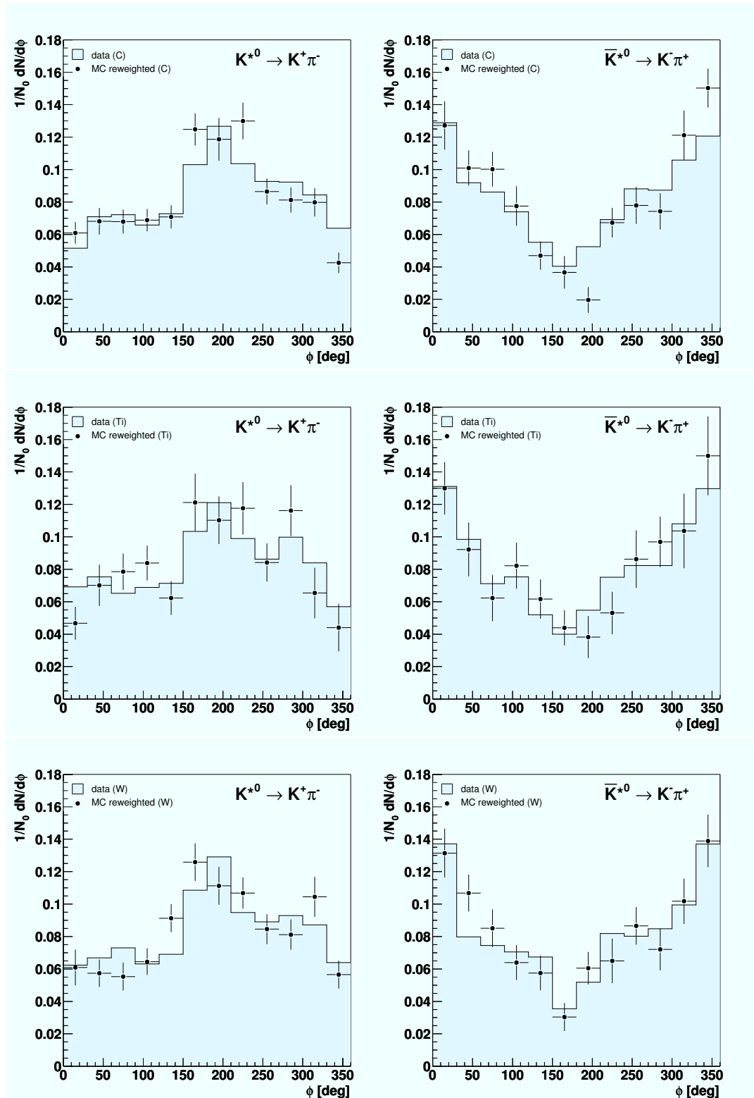
Figure 5.21: Comparison of reconstructed azimuthal distributions in data and Monte-Carlo in the accessible phase space. The distributions are normalized to the same number of entries.
