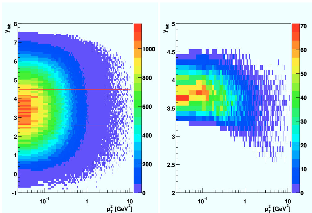
Figure 5.10: Monte-Carlo distributions of K^{*0} production in the p_T^2 - y plane. Left: Generator distribution showing the full phase space of the decay. The y -range accessible by HERA-B is indicated by the horizontal lines. Right: Distribution of reconstructed K^{*0} after application of all selection cuts. Clearly, rapidity and transverse momentum are not independent of each other any more.
