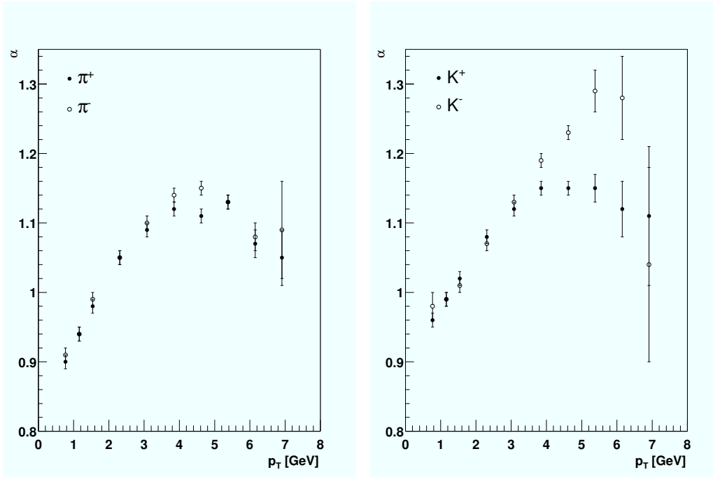
Figure 2.6: Atomic number dependence for the production of \pi^\pm (left) and K^\pm (right) as a function of p_T . For p_T > 1.5 GeV \alpha exceeds one. Figures based on data from [cro77].
