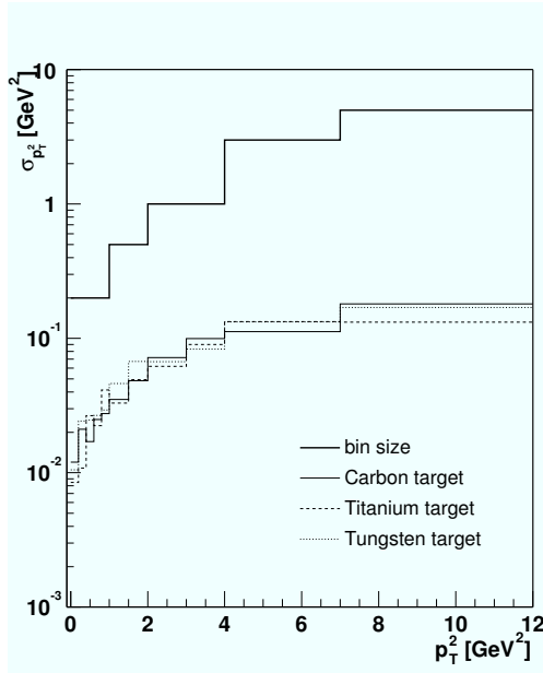
Figure 5.6: Monte-Carlo estimation of the p_T^2 resolution \sigma_{p_T^2} as a function of p_T^2 . The bin widths are superimposed, indicating that in each bin the resolution is much better than the corresponding bin width.
