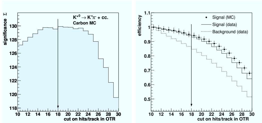
Figure 4.9: Left: K^{*0} signal significance as a function of the cut on the number of hits in the outer tracker. The signal yield used to calculate the significance is derived from the Monte-Carlo simulation, the background comes from real data. The cut of at least 18 hits/track chosen for this analysis is indicated by the arrow. Right: Efficiencies of signal and background as a function of the cut. The data points represent the signal efficiencies obtained from the Monte-Carlo simulation. Both plots are based on the carbon data sample.
