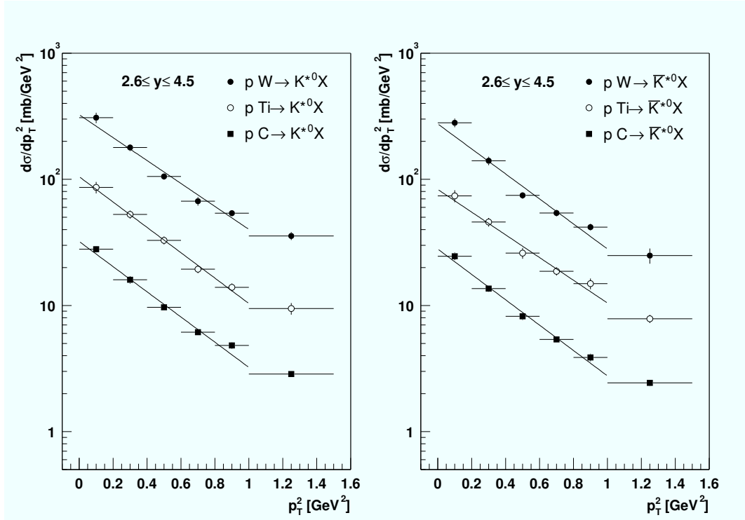
Figure 6.4: Exponential fits to the low- p_T^2 region of the cross section measurements. The onset of flattening beyond p_T^2 = 1 \text{ GeV}^2 is clearly seen.
