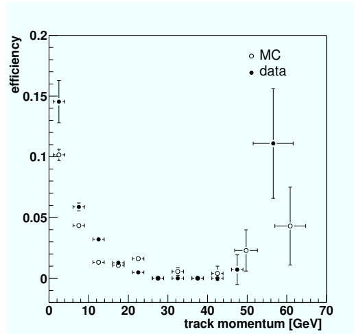
Figure 4.8: Efficiency to mis-identify a true pion as a kaon, derived from K_s^0 \rightarrow \pi^+ \pi^- decays (both for Monte-Carlo and real data). Based on [sta04].
