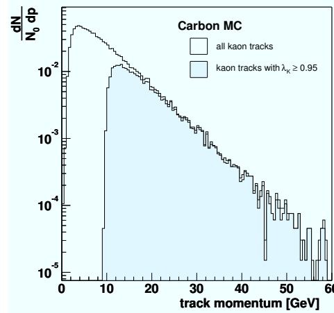
Figure 4.6: Momentum distribution of reconstructed (and matched) kaons. The shaded histogram shows tracks with a kaon likelihood \lambda_K \geq 0.95 . The intrinsic momentum cut at 9.6 GeV is clearly visible.
