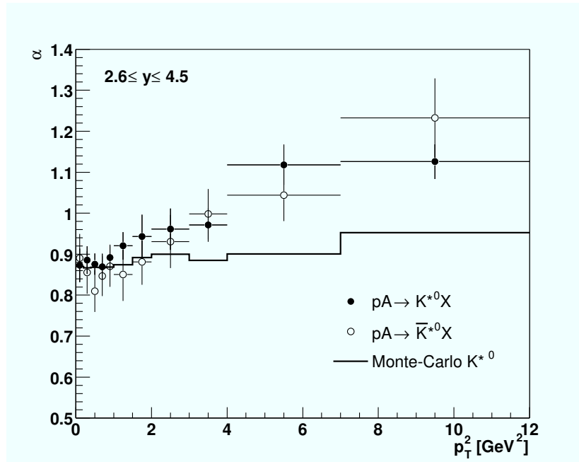
Figure 6.8: Atomic number dependence of the differential production cross sections as a function of p_T^2 .
