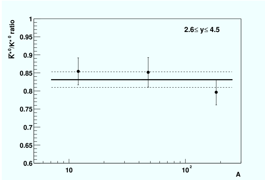
Figure 6.1: Ratio between the \bar{K}^{*0} and K^{*0} production cross sections at mid-rapidity for the different target materials. The horizontal lines indicate the average and the RMS of the results.
