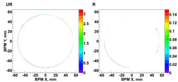
Figure 5: The signal (in V/nC) from a diamond (right) and a sapphire (left) as a function of the beam position. The beam position has been calculated on the basis of the reading from the BPM corrected with the theoretical deflection of the beam by the sweeper magnet. The bunch charge is 1 nC.
