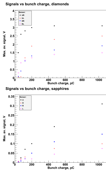
Figure 6: Signal from all diamonds (top) and all sapphires (bottom) as a function of the bunch charge in the machine.
