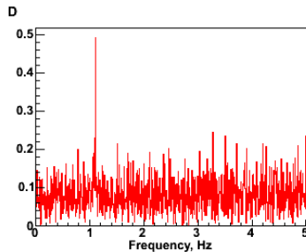
Figure 4: The signal from a sapphire sensor in frequency domain.
