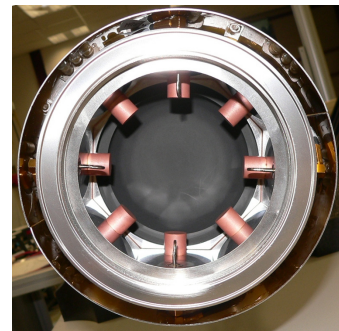
Figure 1: View of the BHM from the dump. The BHM sensors are inside the caps. Four loops of the magnetic-coupled BPM are right in front of the BHM sensors.
