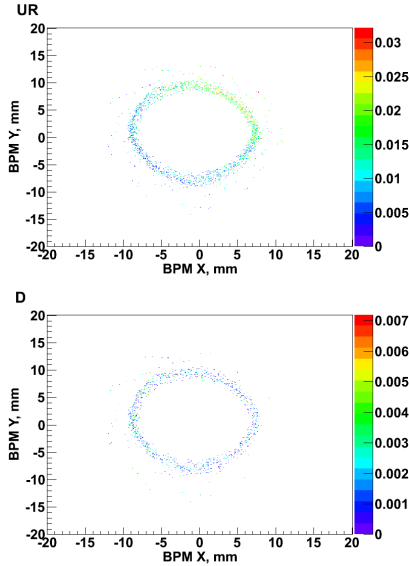
Figure 3: The signals (in V/nC) from a diamond (top) and a sapphire (bottom) sensor as a function of the beam positioning the azimuthal plane (as measured by the BPM). The bunch charge is 500 pC.
