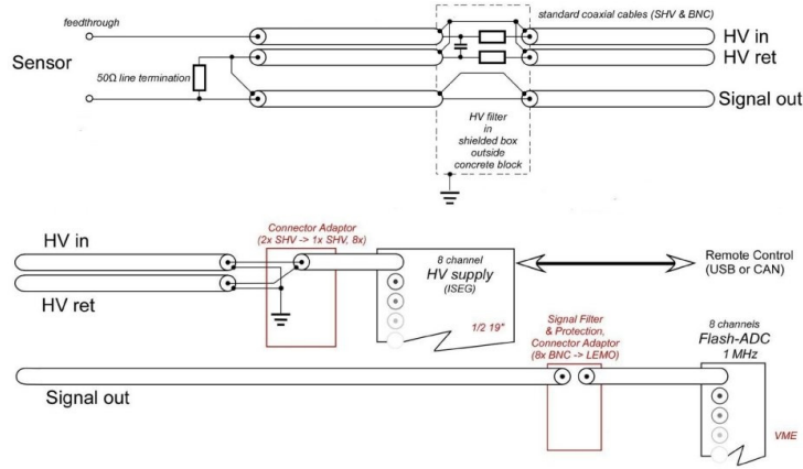
Figure 2: The bias voltage feed and signal readout scheme for each BHM sensor.
