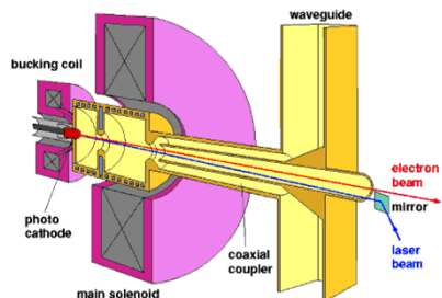
Laser-driven rf gun
