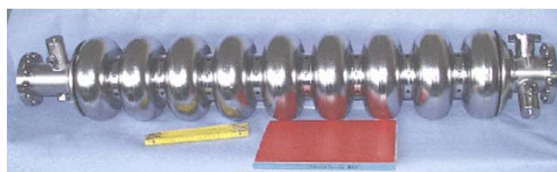
1.3 GHz, Nb, operates at 2 K,
