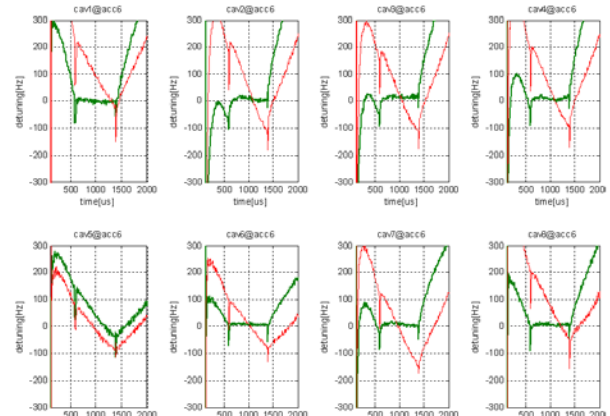
Figure 4: LFD compensation in 6 th accelerating module (green - detuning with piezo compensation, red - without)
