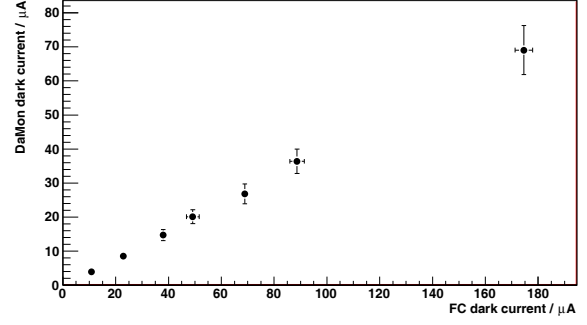
Figure 3: Dark current taken with the DaMon as a function of results with the Faraday Cup.
