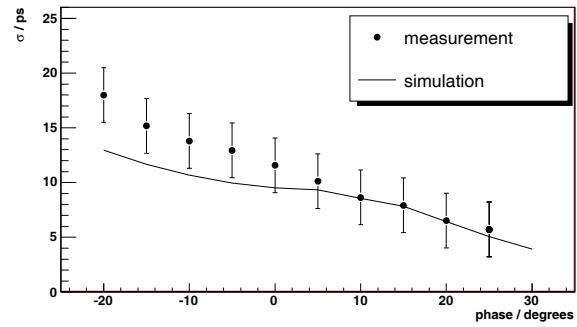
Figure 7: Bunch length measured using Aerogel and a streak camera as a function of injector phase including simulation results. The Aerogel position is 4 m downstream of the DaMon.
