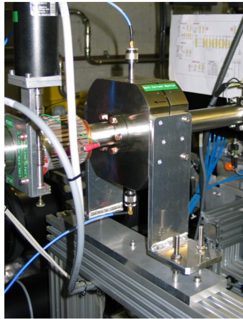
Figure 1: Dark current Monitor at the photo injector test facility.
