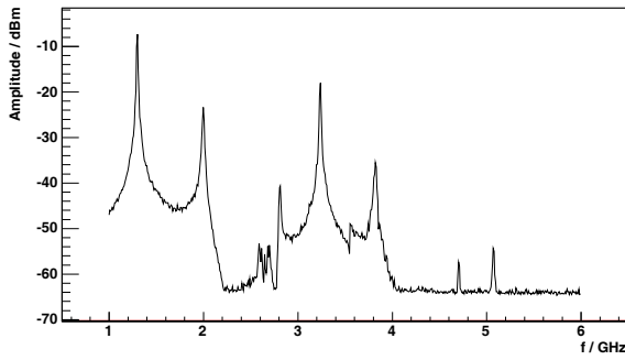
Figure 5: Beam spectrum of the DaMon.
