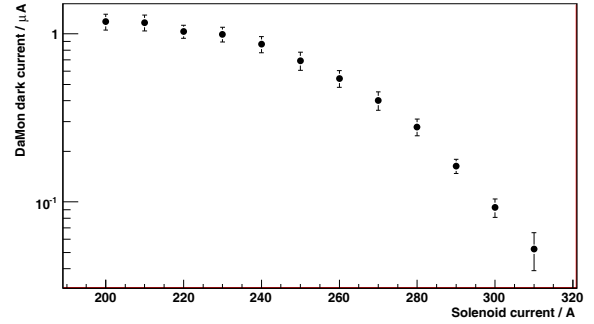
Figure 4: Dark current taken with the DaMon as a function of the injector solenoid current.
