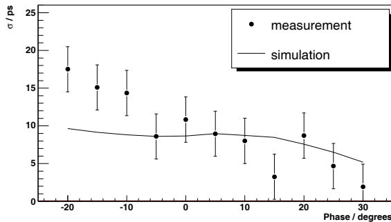
Figure 6: Bunch length measured using the first and third monopole mode from the DaMon signal as a function of injector phase including simulation results.
