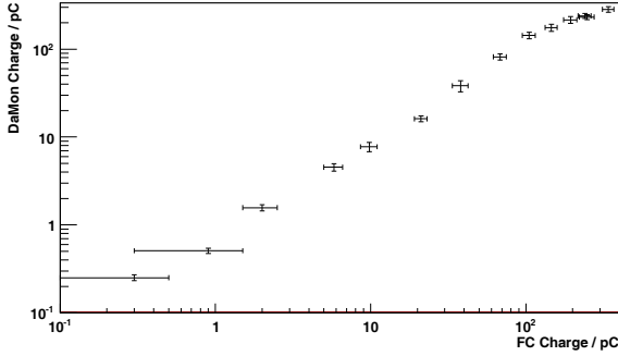
Figure 2: Beam charge taken with the DaMon as a function of results with a Faraday Cup (FC). Error bars are standard deviations of several measurements.
