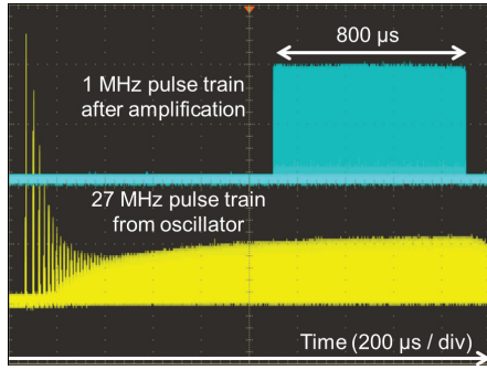
Figure 2: Oscilloscope traces of the laser pulse train of the oscillator (yellow trace), and after final amplification (blue) measured with photodiodes.
