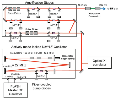
Figure 1: Schematic overview of the laser system.
