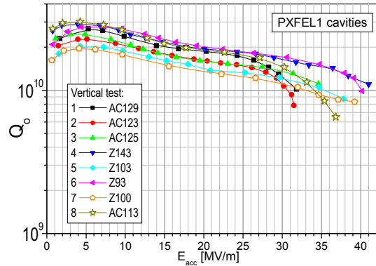
Figure 5: Vertical test results.
