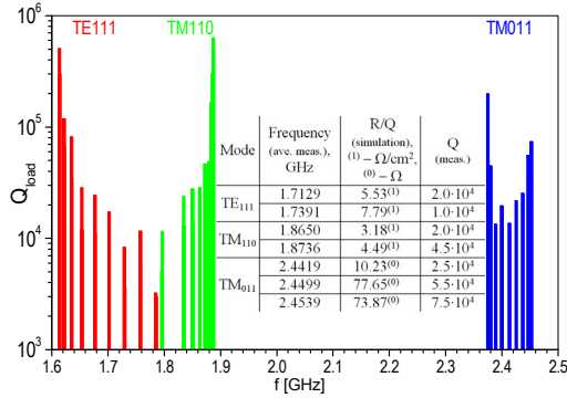
Figure 6: HOMs spectrum.
