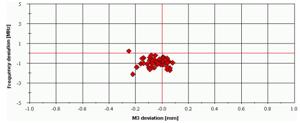
Figure 1: Statistic data for half-cells.
