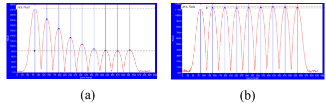
Figure 2: Field distribution of fundamental mode TM010 (a) – before and (b) – after the tuning.
