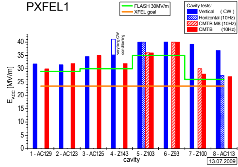
Figure 7: Cavities tests results for module PXFEL 1.
