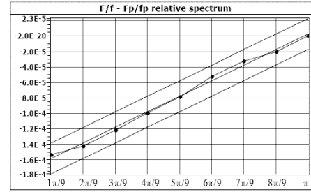
Figure 3: Comparison of spectra for cavity AC158.
