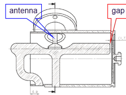
Figure 4: HOM couplers filter tuning.
