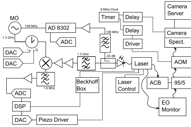
Figure 2: Experimental setup with schematic plan of RF synchronization.
