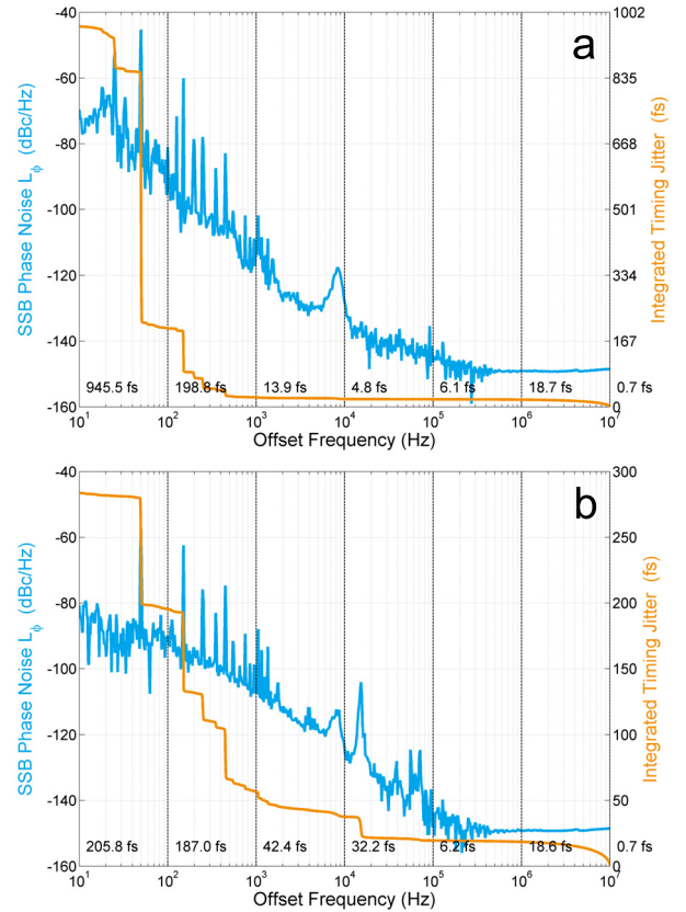
Figure 5: Phase noise and integrated timing jitter with regulation off (a) and regulation on (b).
