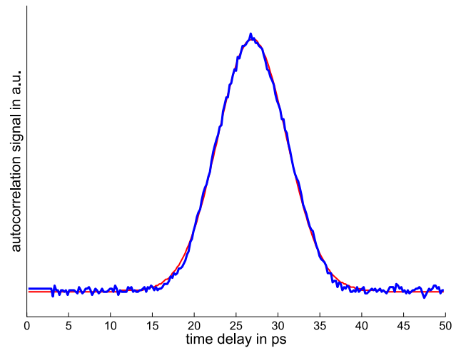
Figure 3: Auto correlating fuction of laser pulses (blue) and Gaussian fit (red) FWHM width of 10.16 ps.
