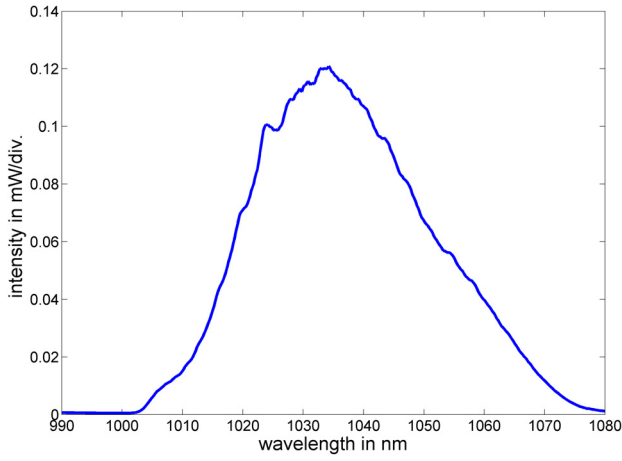
Figure 4: Optical spectrum of pre-amplified laser pulses.
