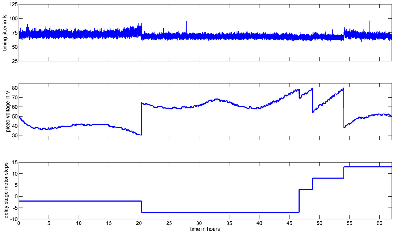
Figure 6: RF synchronization measurement of in-loop timing jitter, piezo voltage and motor position of delay stage for a period of 62 hours.
