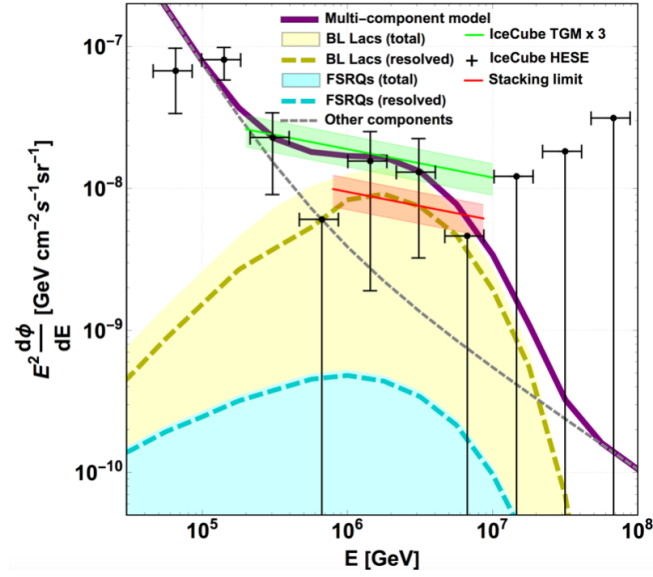
Figure 3: Diffuse neutrino spectrum in IceCube estimated for the baryonic loadings shown in Fig. 2. The black points represent the all-flavor fluxes of IceCube high-energy starting events (HESE, [21]), the green line represents the throughgoing muon flux (multiplied by 3 to account for all three neutrino flavors, [22]) and the red line represents the IceCube stacking limit on the blazar contribution [6]. The shaded yellow and cyan represent the contribution of BL Lacs and FSRQs, respectively, to the total flux of neutrinos, whereas the dotted yellow and cyan curves denote the contribution from resolved sources only. The purple solid curve represents the total neutrino flux expected from blazars. In this case most of the flux is powered by resolved sources, particularly FSRQs.
