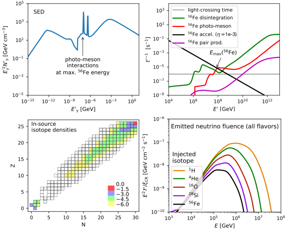
Figure 1: Results of a simulation of the photo-hadronic processes taking place in a blazar jet with luminosity L_\gamma = 10^{48.5} erg/s, considering the acceleration of iron-56. Upper left: time-independent SED, adopted from the Fermi blazar sequence [8]. Upper right: interaction rates of relevant radiative processes. Lower left: energy densities of nuclear isotopes, normalized to the injection luminosity. Lower right: all-flavor neutrino fluence emitted during a flare for the case of different injected isotopes, from protons to iron-56. Neutrino fluences shown in the observer's frame for redshift z = 1 . Figures adapted from [5] and [7].
