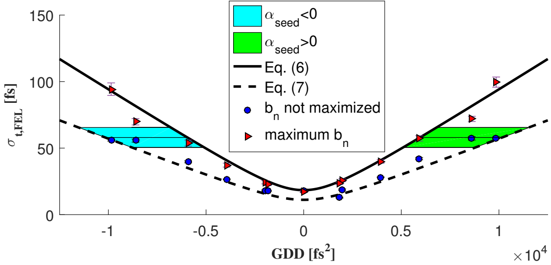
Figure 2: Duration of the seeded FEL pulses \sigma_{t,FEL} as a function of the GDD of the seed laser pulse GDD_{seed} . The color-filled boxes represent the regions where the experimental point was measured from the THz streaking experiment. These boxes are limited vertically from error bars given by the experimental uncertainty and the horizontally from the two theoretical curves. The measured time duration of the FEL pulse permits to retrieve the initial GDD of the seed laser pulse at the beginning of the modulator. The markers represent the FEL performance foreseen from the simulations: red triangles show the case of optimized bunching and the blue circles show the case with small dispersion, so low bunching factor.
