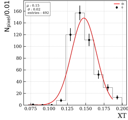
Figure 7: Crosstalk probability distribution for one third of the camera
