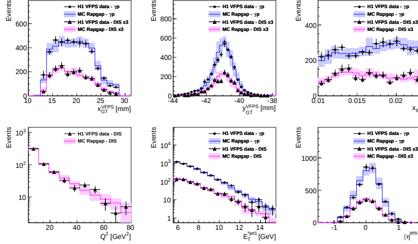
Figure 2: Control distributions of selected reconstructed quantities.
