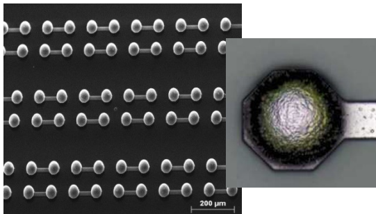
solder ball placement
