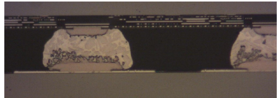
after flip chip bonding
