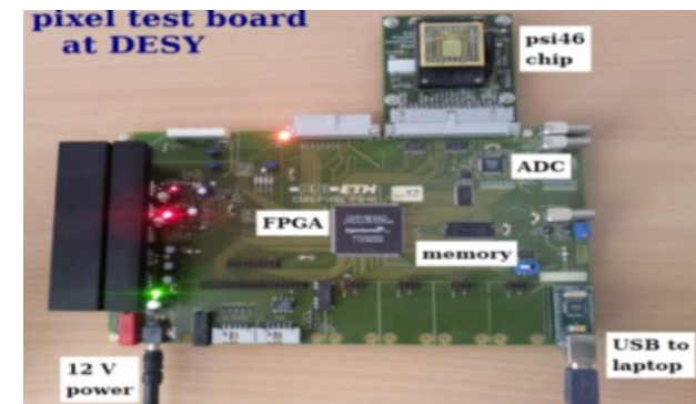
Test Board
