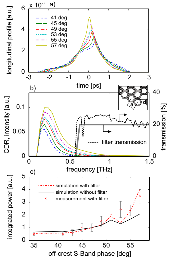
Figure 4: For different electron bunch compressions, the longitudinal bunch profile for 65 pC and 200 MeV is measured with the TDC a). Therewith, the corresponding CDR spectrum is derived b). Moreover the simulated transmission of a high-pass THz filter is shown in b). The inset illustrates the air filled hole array in a thick copper plate, used as the highpass THz filter ( a=600\ \mu\text{m} , d=300\ \mu\text{m} ). The resulting characteristic of the spectrally integrated signal as a function of the electron bunch compression angle is depicted in c). This data was taken without X-band.
