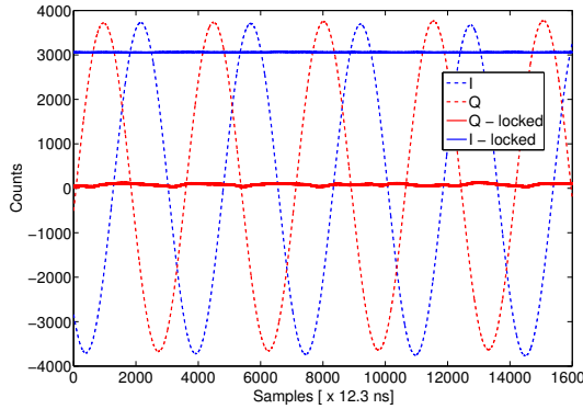
Figure 5: I and Q detected in the digitizer SIS8300-L board.
