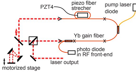
Figure 2: Simplified schematic of the Yb-fiber laser.
