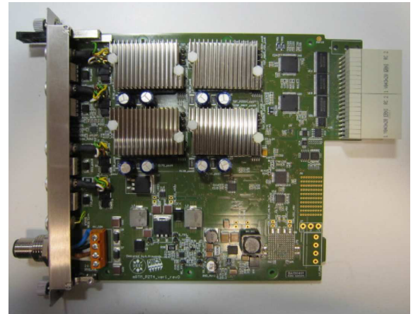
Figure 4: Photograph of the DRTM-PZT4 4-channel piezo driver board.
