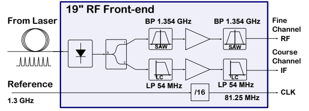
Figure 3: : Block diagram of the RF front-end 19" chassis.
