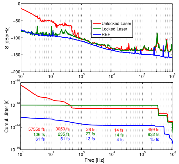
Figure 6: Phase noise (top) and integrated timing jitter (bottom) of the 1.3 GHz reference (blue), free-running laser (red) and locked laser (green). The numbers in the lower plot represent the timing jitter per frequency decade.
