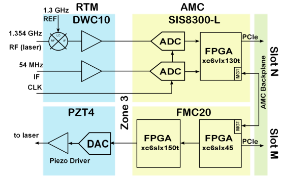
Figure 1: Block diagram of the MTCA.4 board setup.
