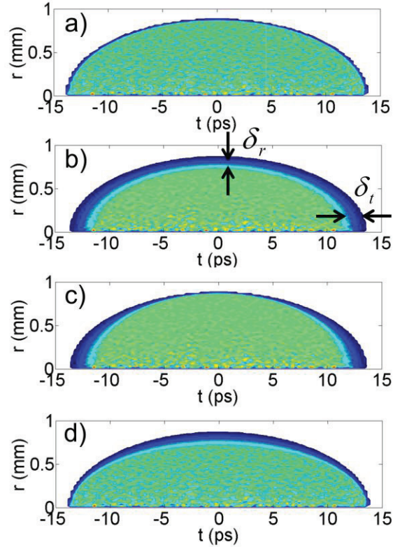
Figure 7: Border sharpness modelling in ASTRA. a) Perfect 3D shape, b) 20 % distortion in temporal and radial directions, c) 20 % distortion only in the temporal direction, d) 20 % distortion only in the radial direction.
