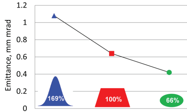
Figure 2: Transverse rms normalized emittance optimized for 3 different laser shapes with the same electron beam rms length at EMSY1.
