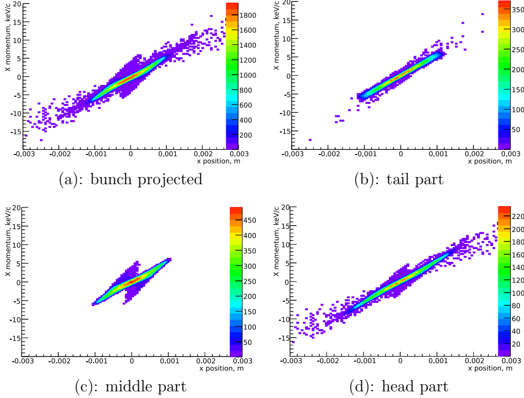
Figure 2.7: A simulated (ASTRA) optimized projected phase space distribution of the bunch and of different parts separately. The full bunch emittance is 0.63 mm mrad; tail - 0.45 mm mrad; middle (highest current) - 0.62 mm mrad; head - 0.75 mm mrad.
