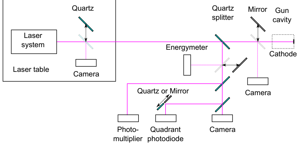
Figure 3.3: A scheme of the laser transverse profile and intensity diagnostics.
