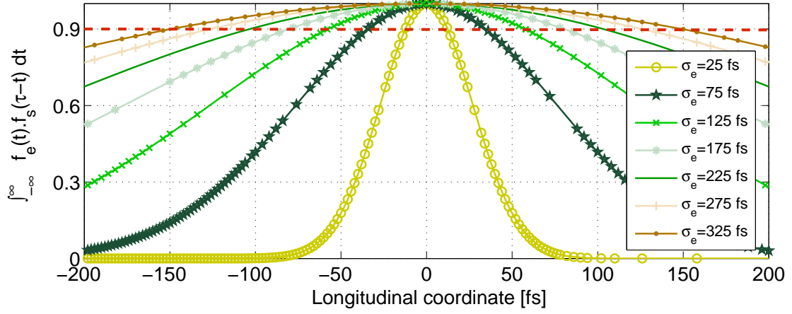
Figure A.2: The convolution of electron bunch and seed pulse distribution for different electron bunch duration. The rms seed pulse duration is \sigma_s = 10 fs. The optimum overlap is defined for the convolution functions \geq 0.9 .
