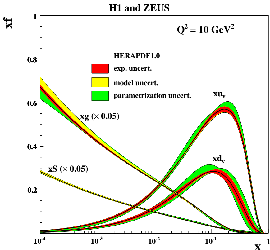
Figure 2.4: The parton distribution functions from HERAPDF1.0, xu_v , xd_v , xS = 2x(\bar{U} + \bar{D}) , xg , at Q^2 = 10 \text{ GeV}^2 . The gluon and sea quark distributions are scaled down by a factor 20 [28].
