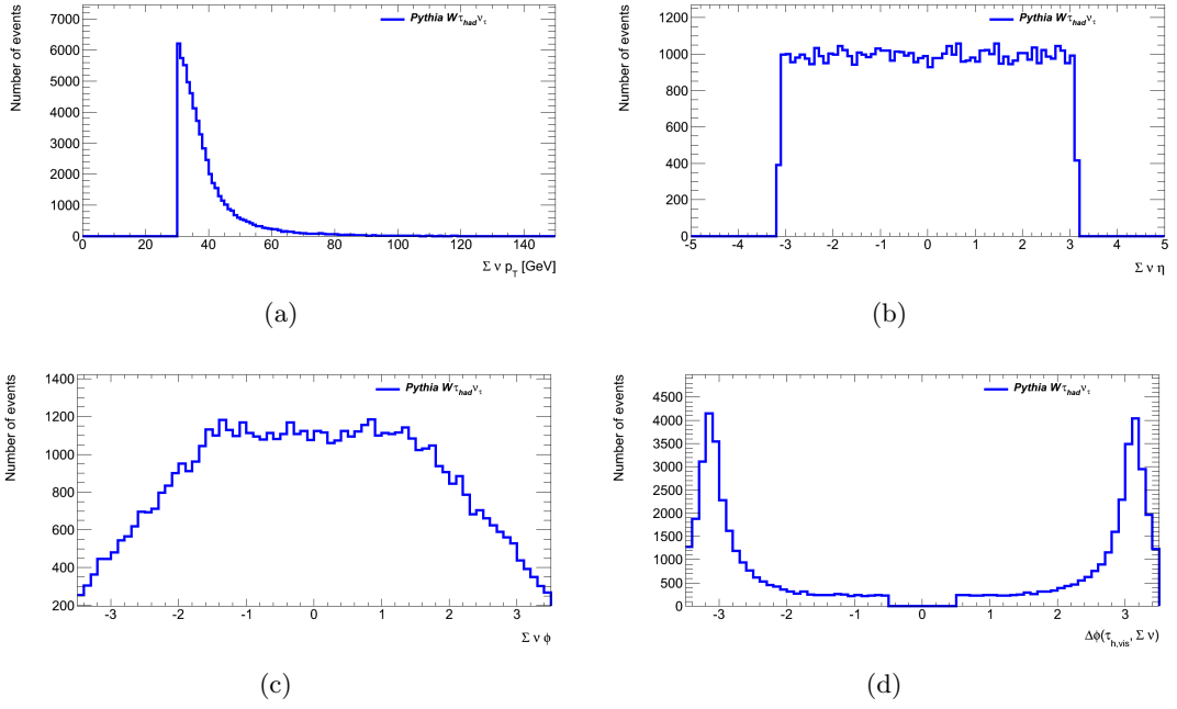
Figure B.8: (a) Transverse momentum, (b) pseudorapidity \eta , (c) angle \phi of the sum of the neutrinos \Sigma \nu , and (d) angle \Delta\phi between the true \tau_{h,vis} lepton and the sum of the neutrinos \Sigma \nu after all cuts on the transverse momentum p_T and the pseudorapidity \eta of the true \tau_{h,vis} lepton, the transverse momentum of the sum of the neutrino (\Sigma p^\nu)_T and the |\Delta\phi(\tau_{h,vis}, \Sigma \nu)| .
