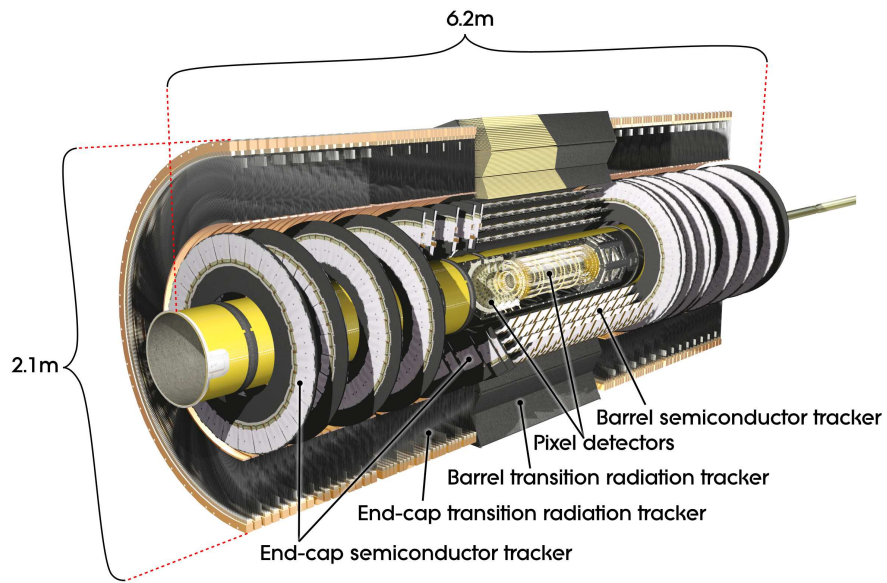
Figure 3.6: Cut-away view of the ATLAS Inner Detector [58].
