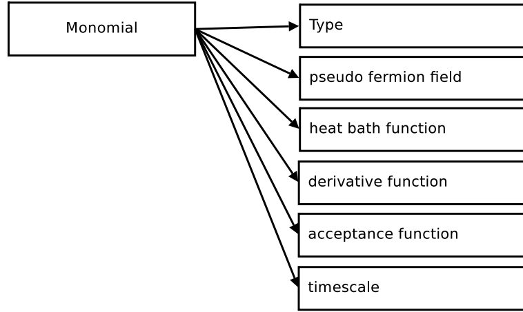
Fig. 5. Data type monomial and its components.
