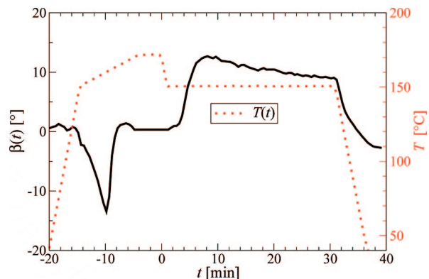
Figure 4. Tilt-angle tracking curve, \beta(t, T) , from the automatic fiber mapping procedure in an experiment with long exposure of the patterns (20 s) in which \beta changes considerably (HEPP; melt annealing at 171 °C and recrystallization at 150 °C).
