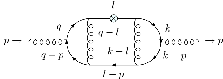
Figure 19: Example 3-loop graph
