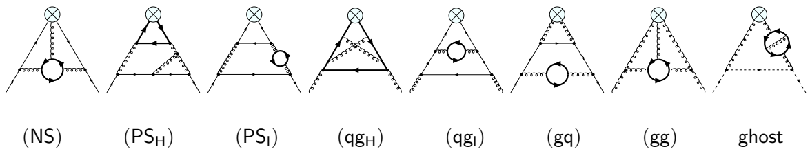
Figure 10: Examples for 3-loop diagrams contributing to the massive operator matrix elements: NS - non-singlet, PS_{H,l} - pure-singlet, singlet qg_{H,l} , gq , gg and ghost contributions. Here the coupling of the gauge boson to a heavy or light fermion line is labeled by H and l, respectively. Thick lines: heavy quarks, curly lines: gluons, full lines: quarks, dashed lines: ghosts.
