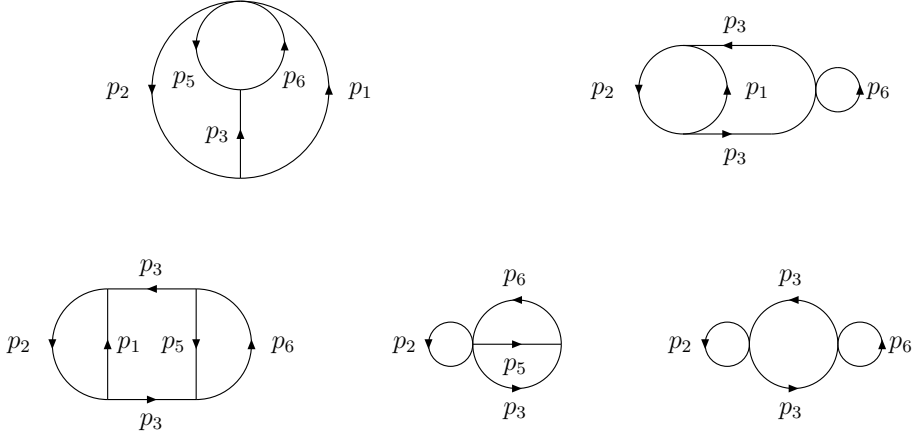
Figure 16: Additional 3-loop topologies for MATAD.
