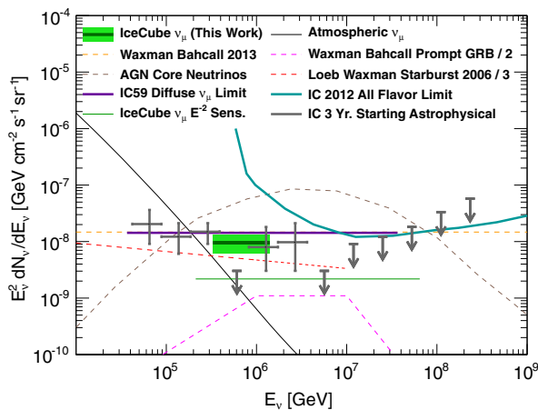
FIG. 4 (color online). Comparison of the best-fit per-flavor astrophysical flux spectrum of E^{-2} from this work, assuming a flavor ratio of 1:1:1 (shown in dark green with the 68% error range in lighter green) to other selected IceCube measurements (heavy lines) [4,12] and theoretical model predictions (thin dashed lines) [5–7,17,20,28]. The sensitivity of this analysis is also shown as the thin green line.
