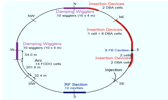
Figure 1: Present layout of Petra III
