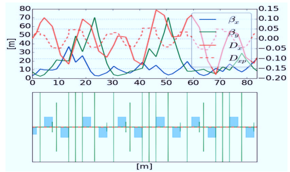
Figure 7: Bunch decompressor optics, for R_{56} = -10 cm and \mathcal{I}_5 = 2 \cdot 10^{-6} \text{ m}^{-1}
