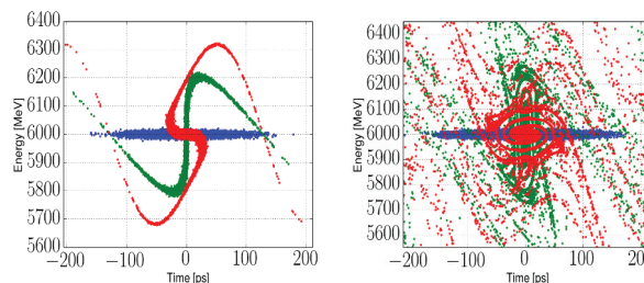
Figure 4: Effect of a map with both R_{56} positive, 3.9 GHz. Initial longitudinal phase space distribution is shown in blue, the compressed and the decompressed distributions are shown in green and red. Left: effect of one turn. Right: effect of 1000 turns.
