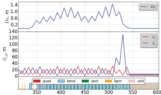
Figure 6: Upstream arc and undulator section optics. In the undulator section \langle\beta_X\rangle = \langle\beta_Y\rangle = 5 m. All optics calculations in the paper are done with OCELOT [3].
