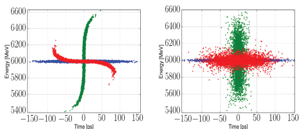
Figure 3: Effect of a map with both R_{56} positive, 1.3 GHz. Initial longitudinal phase space distribution is shown in blue, the compressed and the decompressed distributions are shown in green and red. Left: effect of one turn. Right: effect of 1000 turns.
