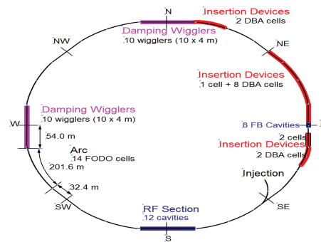
Figure 1: Present layout of Petra III
