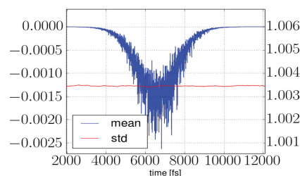
Figure 5: Mean relative energy loss (blue, left axis) and rms relative energy spread (red, right axis) in units of 10^{-3} inside the electron bunch after the undulator for 20x compression, with approx. 50MW peak power. The energy spread includes the initial energy spread of 10^{-3} .
