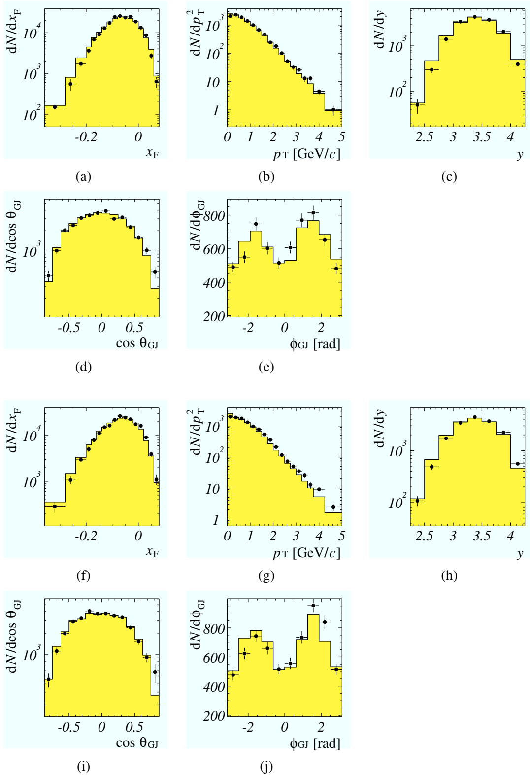
Figure D.3: J/\psi kinematics in data (points) and MC simulation (histograms) for the wire combination I112. (a)–(e) x_F , p_T , y , \cos \theta_{GJ} , and \phi_{GJ} for J/\psi produced on the wire Inner II. (f)–(j) x_F , p_T , y , \cos \theta_{GJ} , and \phi_{GJ} for J/\psi produced on the wire Inner I. The MC distributions are scaled to the integral of the data distributions.
