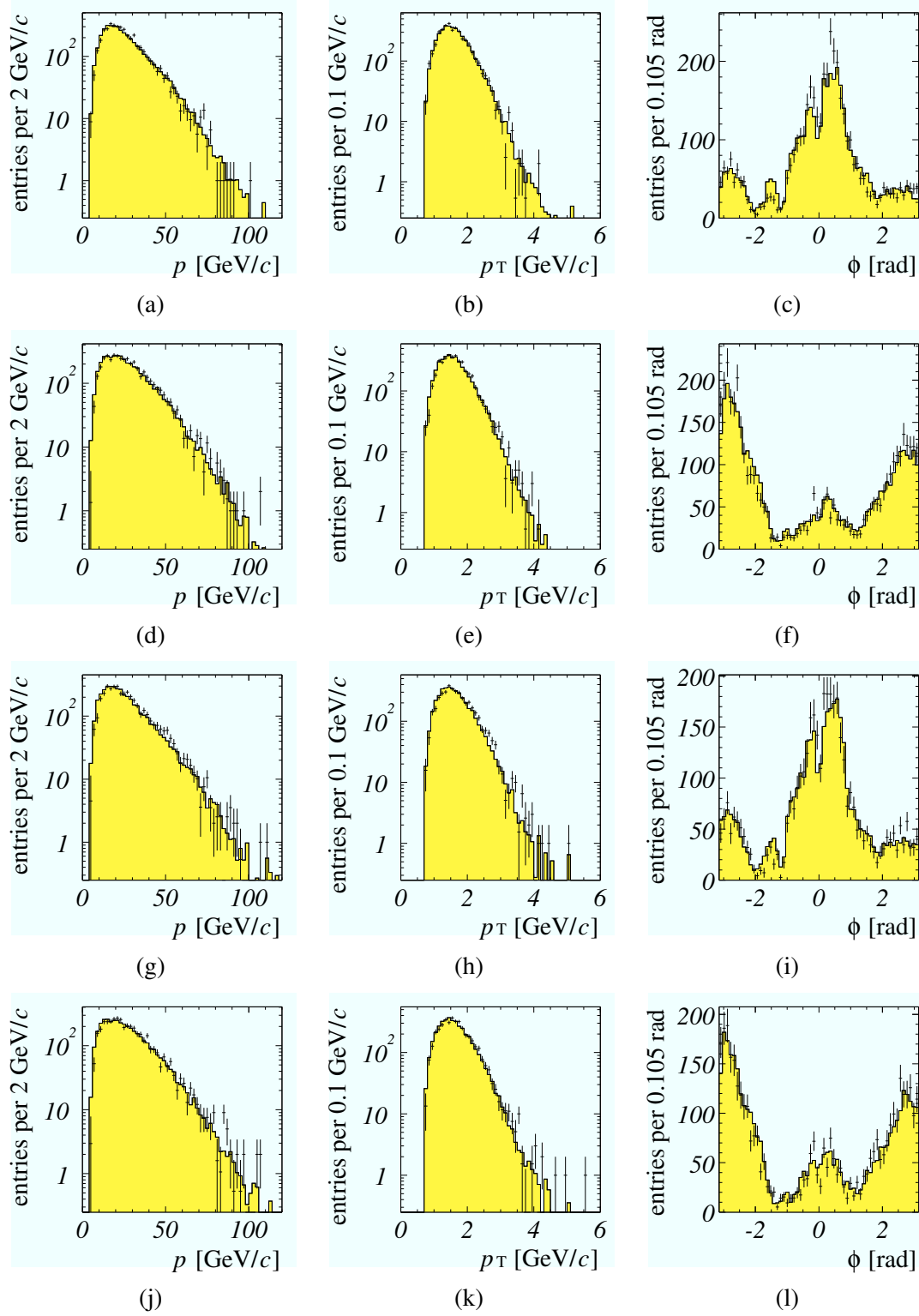
Figure D.1: Kinematics of muons from J/\psi decays in data (points) and MC simulation (histogram) for the wire combination I1I2. (a)–(c) p , p_T , and \phi of \mu^+ produced on the wire Inner II. (d)–(f) p , p_T , and \phi of \mu^- produced on the wire Inner II. (g)–(i) p , p_T , and \phi of \mu^+ produced on the wire Inner I. (j)–(l) p , p_T , and \phi of \mu^- produced on the wire Inner I. Background is removed via sideband subtraction, and the MC distributions are scaled to the integral of the data distributions.
