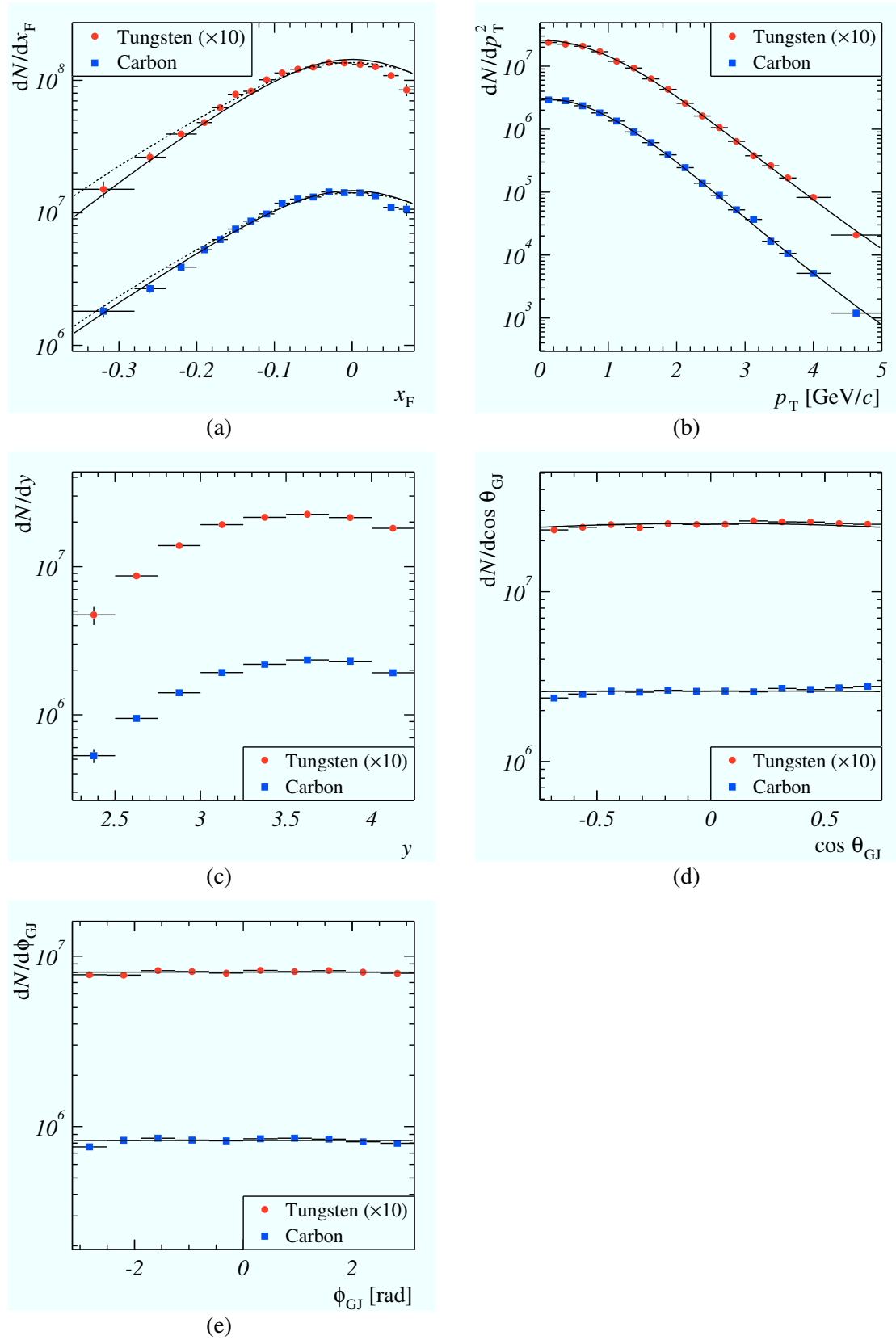
Figure 4.14: J/\psi differential distributions summed over all data sets. (a) x_F distributions fitted with a parametrization of the E75 fit (solid line) and the NRQCD prediction (dashed line). (b) Fit to p_T distributions. (c) y distributions. (d) Fit to \cos \theta_{GJ} distribution. (e) Fit to \phi_{GJ} distribution. All distributions obtained from tungsten wires are scaled by a factor of 10. The fit results are summarized in Tables 4.9 and 4.10.
