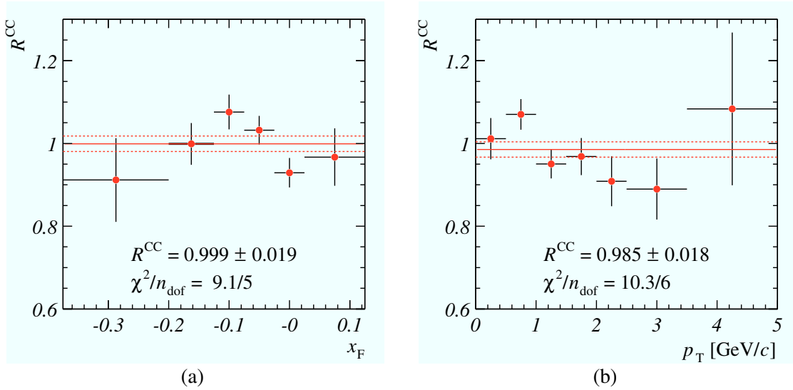
Figure 6.6: Average cross section ratio R^{\text{CC}} measured in the control sample from the wire combination B112 in the calibration period of January 2003 (II). (a) x_F dependence. (b) p_T dependence. The lines indicate the central values and statistical uncertainties of fits to the distributions with a constant. The y-scales are zero-suppressed.
