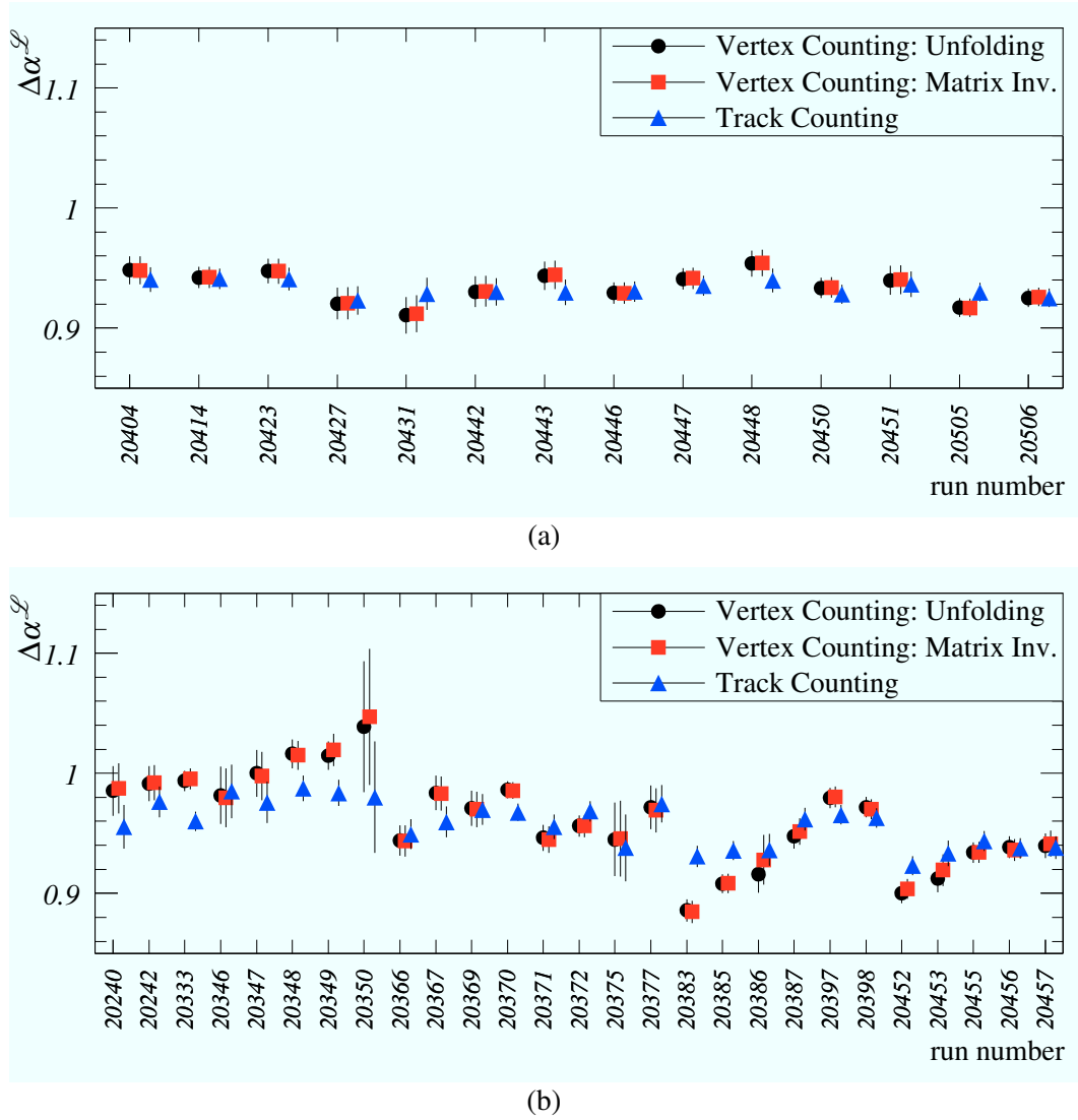
Figure 5.1: Comparison of the luminosity ratios obtained by the vertex counting method and the track counting method. The figures show the shift in the nuclear suppression parameter \alpha for luminosities determined by the methods of matrix inversion and Bayesian unfolding and for luminosities determined by the track counting method. (a) Runs taken with the wire combination III2 in the calibration period of November 2002. (b) Runs taken with the wire combination in I1B1 in November 2002.
