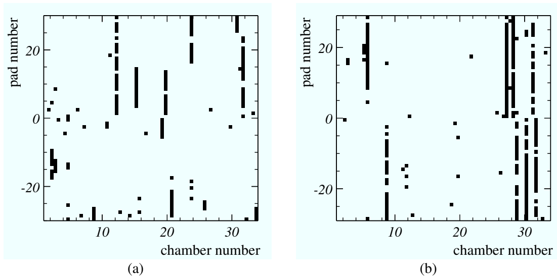
Figure A.3: Masks for defective channels in the muon pad system for the November 2002 calibration period for (a) MU3 and (b) MU4. The shaded areas represent pads masked in the MC simulation. The chambers are numbered according to the scheme described in [Har99].
