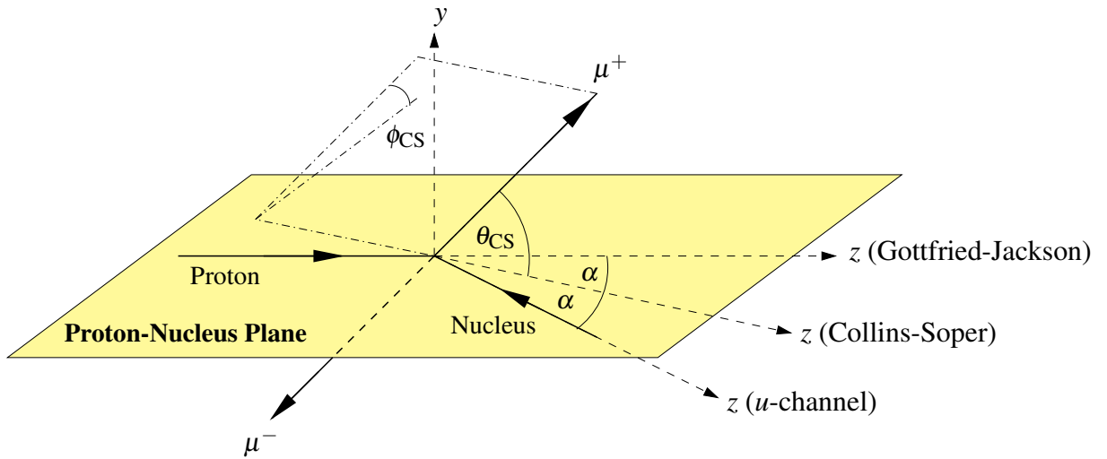
Figure B.2: Definitions of angular variables in the decay J/\psi \rightarrow \mu^+ \mu^- , given in the rest frame of the J/\psi (after [Con89]). The different choices for the coordinate system are described in the text.
