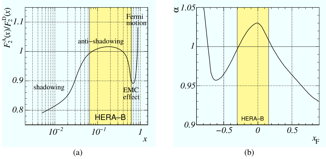
Figure 3.6: Illustrations of charmonium suppression by nuclear structure functions: (a) Schematic drawing of the structure function ratio F_2^A(x)/F_2^D(x) (after [Arn94]). The features of the ratio are explained in the text. (b) Charmonium suppression parameter \alpha(x_F) due to nuclear PDFs. The calculation is performed for 800 GeV beam energy using the EKS98 set of nuclear PDFs (after [Vog00]). The x - and x_F -ranges covered by HERA-B are indicated by the shaded areas.
