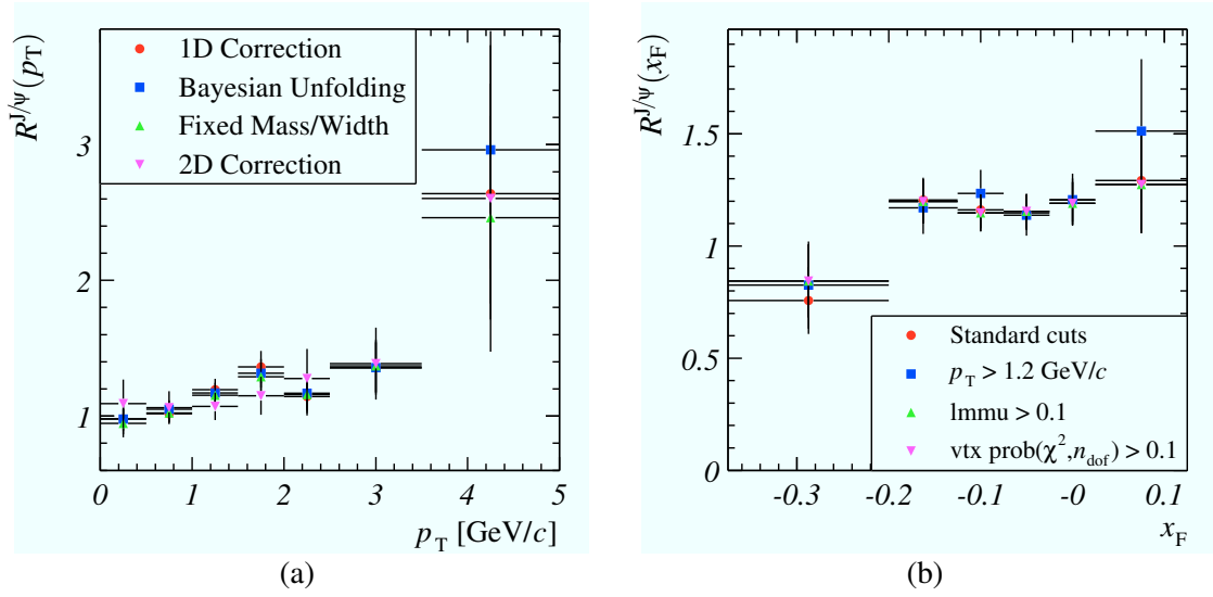
Figure 6.3: Systematic checks of J/ψ yield ratios for the wire combination I1B1 in the calibration period of November 2002. (a) Yield ratio as a function of p_T , variation of efficiency correction method. (b) Yield ratio as a function of x_F , variation of event selection cuts.
