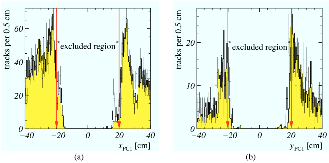
Figure 4.3: Fiducial cuts in the OTR superlayer PC1. Muon tracks from J/\psi candidates which could be fitted to a vertex with an invariant mass in the range of 3.0\text{--}3.2\text{ GeV}/c^2 are extrapolated to the z -position of PC1. The data points are taken from all runs with the wire combination I1I2 in November 2002, and the histograms show the corresponding results from the MC simulation, scaled to the integral of the data. (a) x -positions of all tracks in the range of |y_{\text{PC1}}| < 10\text{ cm} . (b) y -positions of all tracks in the range of |x_{\text{PC1}}| < 10\text{ cm} . The cut values are indicated by the arrows.
