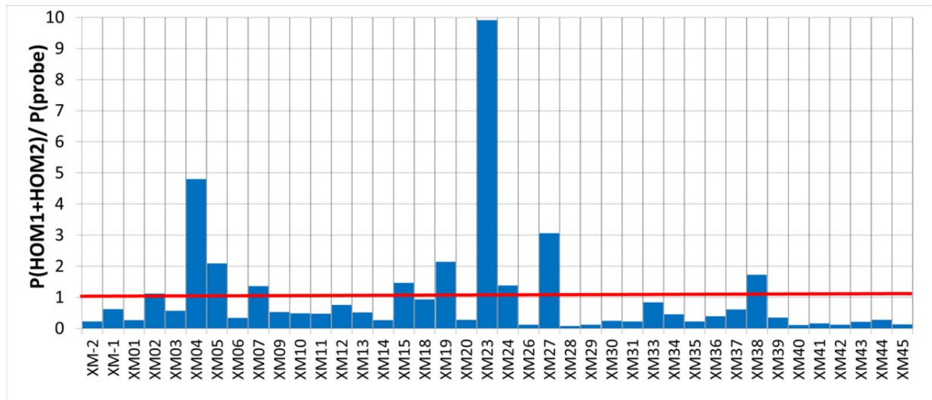
Figure 6: Average ratio P(\text{HOM1} + \text{HOM2}) / P(\text{probe}) for 8 cavities in module
