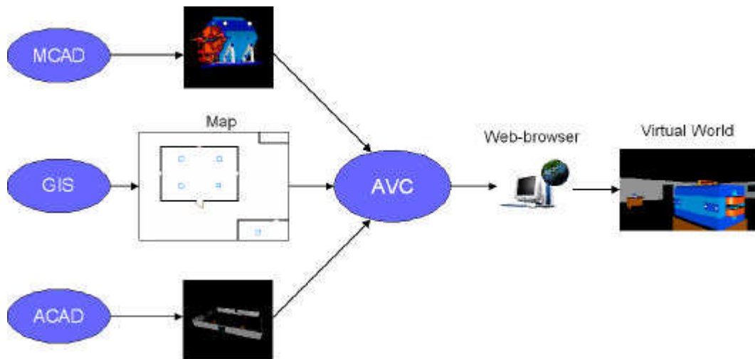
Figure 1-1 High-level AVC structure.
