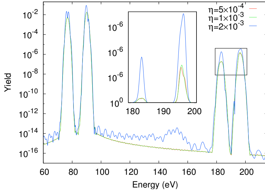
Figure 5.6: The argon photoelectron spectrum along the polarization axis of the field, calculated with t-surff, is shown for a pulse with 105 eV photon energy, 9 \times 10^{13} \text{ Wcm}^{-2} intensity and 1.2 fs duration for different CAP strengths. The radial grid size is r_{\max} = 150 a.u., the CAP radius is r_{\text{CAP}} = 120 a.u., and r_c = 100 a.u. The oscillations are due to reflections from the end of the radial grid and/or the CAP. © 2014 APS
