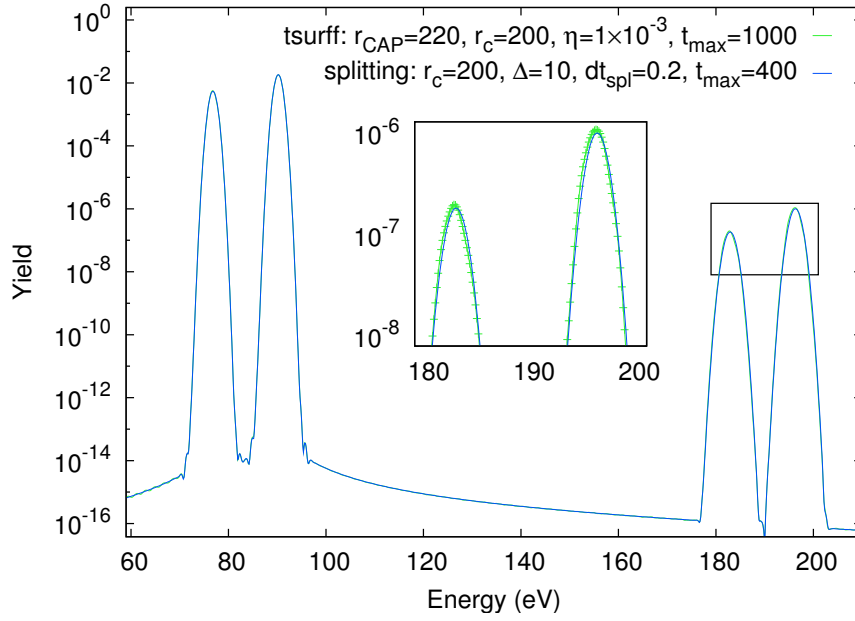
Figure 5.8: The argon photoelectron spectra obtained with the splitting and the t-surff methods for a pulse with 105 eV photon energy, 9 \times 10^{13} \text{ Wcm}^{-2} intensity and 1.2 fs duration along the polarization direction are compared. The radial grid size is r_{\text{max}} = 250 a.u. for both methods. © 2014 APS
