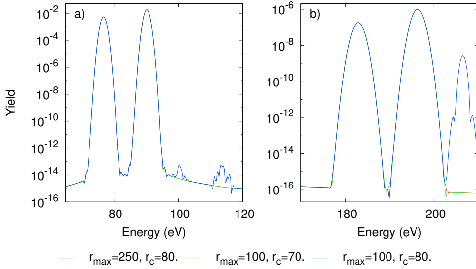
Figure 5.1: The photoelectron spectrum of argon for a pulse with 105 eV photon energy, 9 \times 10^{13} \text{ Wcm}^{-2} intensity and 1.2 fs duration is shown for different radial grid sizes r_{\text{max}} and splitting radii r_c . The smoothing parameter is \Delta = 10 a.u. and the splitting time step is dt_{\text{spl}} = 0.2 a.u. Panel a) shows the one-photon absorption lines, panel b) shows the energetically lowest ATI lines for different splitting radii. All radii are given in atomic units. The spectrum does not change under variation of the splitting radius as long as around 30 a.u. units are left for absorption. © 2014 APS
