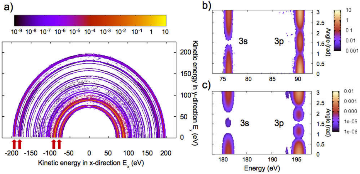
Figure 6.3: a) Angle-integrated PES presented in cartesian coordinates similar to a velocity map image in experiment, the x -axis being the kinetic energy in x direction and the y -axis in y direction. The z axis is defined as the polarization direction of the light. One can distinguish the one-photon peaks and the ATI peaks as circles with the kinetic energy corresponding to the photon energy minus the orbital binding energy, see red arrows. b) Two-dimensional one-photon photoelectron peaks, and c) ATI (bottom) photoelectron peaks of argon for a pulse of 105 eV, a pulse duration of 2.6 fs and an intensity of 10^{15} \text{ Wcm}^{-2} , now as a function of the angle \theta with respect to the polarization direction (top view on the spectra shown in Fig. 5.4). The angular distribution corresponds to a superposition of spherical harmonics belonging to the angular momentum states arising in ionization.
