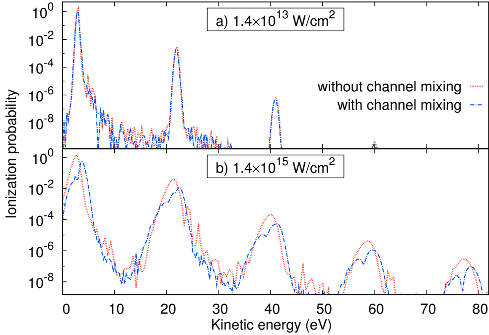
Figure 5.9: Argon photoelectron spectra calculated with the splitting method ( \Delta = 10 a.u., dt_{\text{spl}} = 0.2 a.u., and r_c = 80 a.u.). a) Spectrum calculated for a pulse of 0.7 a.u. photon energy, 4.6 fs duration and an intensity of 1.4 \times 10^{13} \text{ Wcm}^{-2} . The one-photon peak and three ATI peaks are shown. b) Spectrum for the same pulse parameters, except for the intensity, which amounts to 1.4 \times 10^{15} \text{ Wcm}^{-2} . The peaks split when the channel coupling is included in the calculation.
