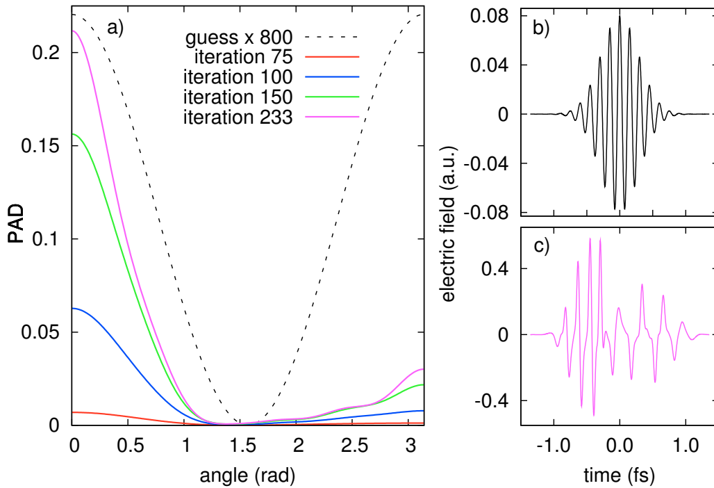
Figure 8.5: Maximization of the difference in emission probability for the lower and the upper hemisphere for hydrogen: a) Energy-integrated PADs are shown for several iterations starting with the initial PAD which is shown magnified by the factor 800 for better visibility (dashed gray line). After 233 iterations the asymmetry is considerably increased. The overall ionization probability is also larger than initially. Although the probability for emission into the lower hemisphere also grows, their difference increases. b) Guess pulse yielding the initial PAD. c) Optimized field obtained with the spectral constraint. Note that the amplitude is significantly larger than for the guess pulse, panel b).
