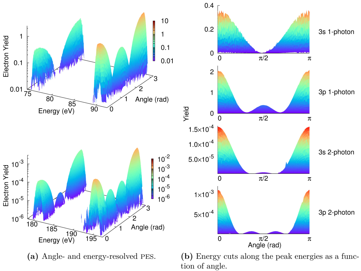
Figure 5.4: The energy- and angle-resolved argon photoelectron distribution produced with the splitting method is shown for an XUV pulse at 105 eV photon energy, 1.0 \times 10^{15} \text{ Wcm}^{-2} intensity and 2.6 fs pulse duration. The grid size is r_{\text{max}} = 100 \text{ a.u.} , r_c = 20 \text{ a.u.} , \Delta = 5 \text{ a.u.} , and dt_{\text{spl}} = 10 \text{ a.u.} The angle denotes the direction with respect to the polarization axis of the pulse. The angular distribution reflects the change in angular momentum by multiphoton absorption. © 2014 APS
